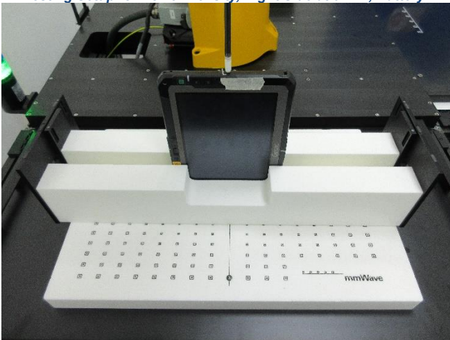
Testing Setup for Power Density, Right Side at 0 mm, Battery1
