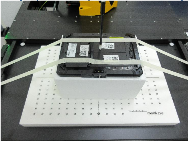
Testing Setup for Power Density, Bottom Surface at 0 mm, Battery1
