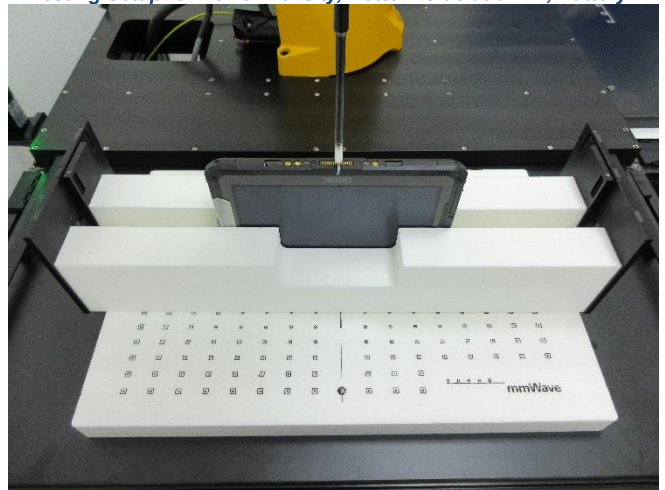
Testing Setup for Power Density, Bottom Side at 0 mm, Battery1
