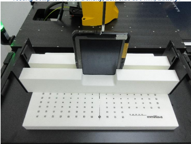
Testing Setup for Power Density, Left Side at 0 mm, Battery1
