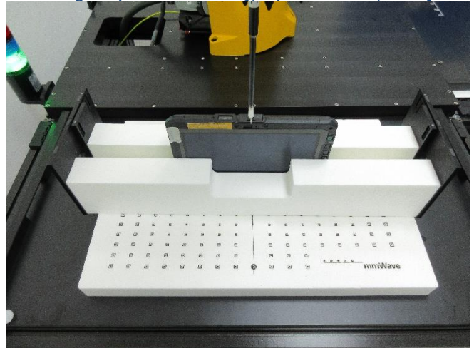
Testing Setup for Power Density, Top Side at 0 mm, Battery1
