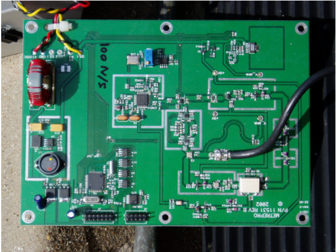
Truck Radio PCB Top
