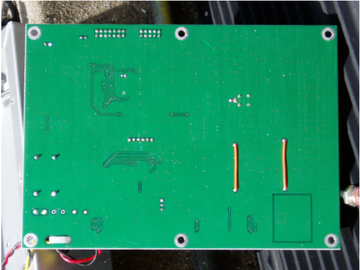
Truck Radio PCB Bottom
