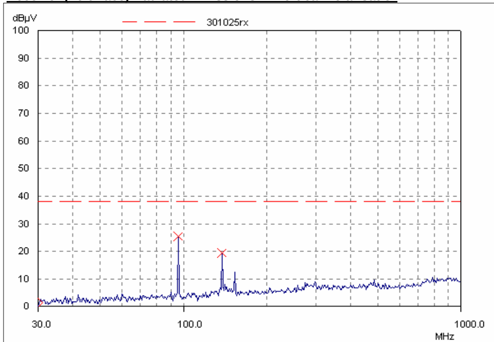
PLOT 13 Receiver (Left Face) Radiated Emissions in Vertical Polarisation
