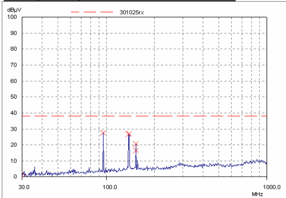
PLOT 13 Receiver (Front Face) Radiated Emissions in Vertical Polarisation
