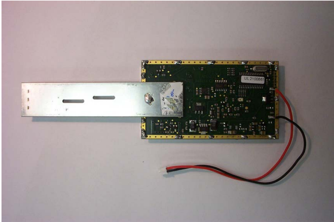
Fig 1: SA50 PCB Assembly – Control Side
