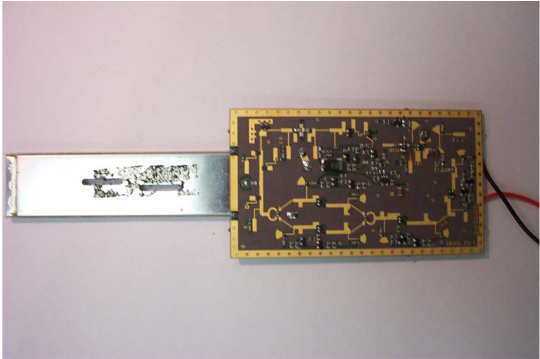
Fig 3: SA50 PCB assembly – RF side with screen removed
