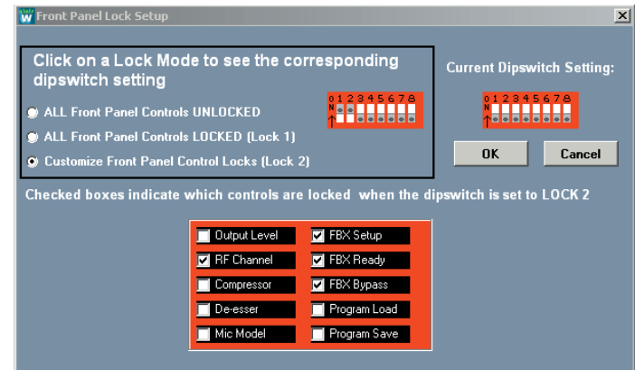
Fig. 13g - Front Panel Lock Setup
