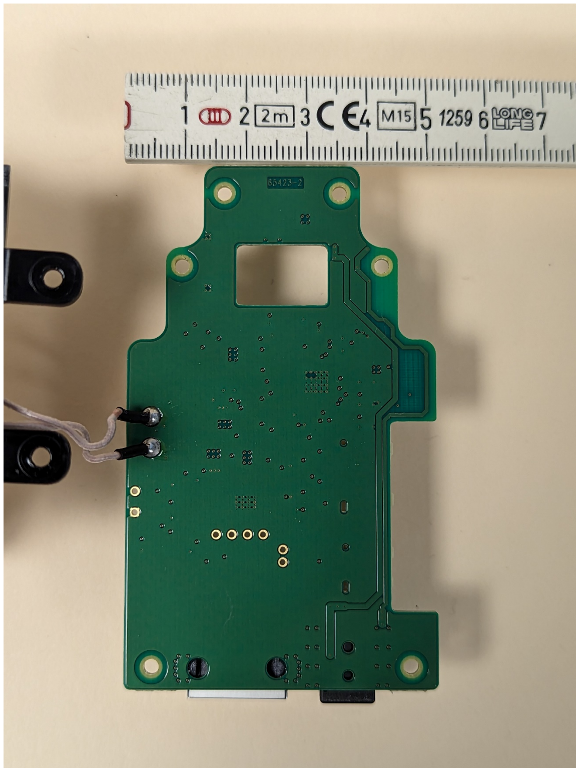
Main PCB Bottom
