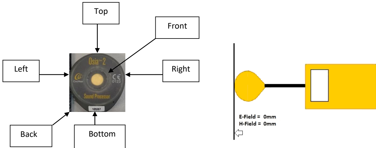
Figure 9: Measurement setup
