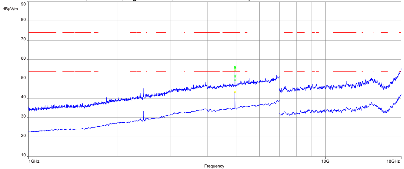
Plot 3: 1 GHz to 18 GHz, TX mode, high channel, vertical & horizontal polarization
