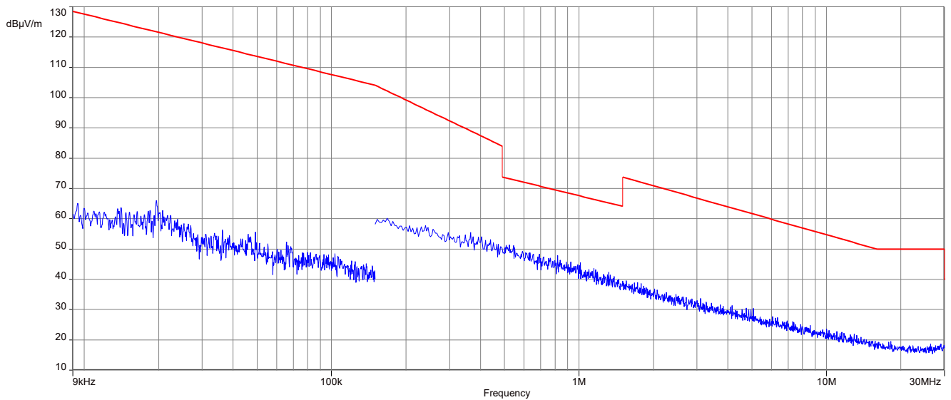
Plot 2: 9 kHz to 30 MHz, mid channel, transmit mode
