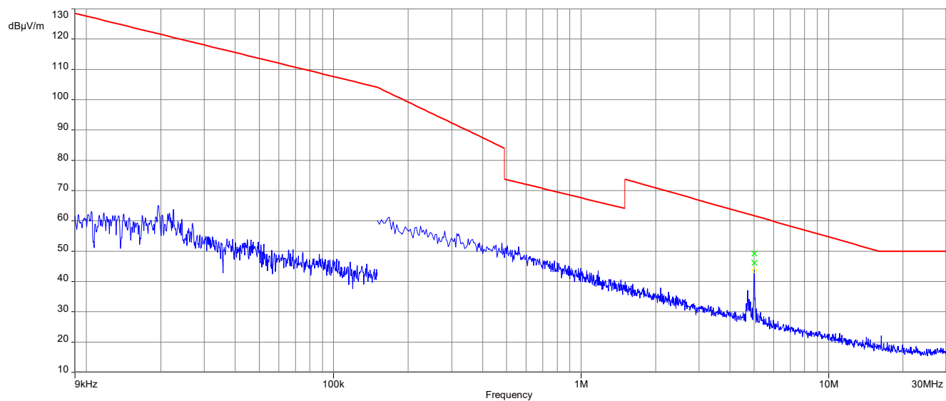
Plot 3: 9 kHz to 30 MHz, high channel, transmit mode
