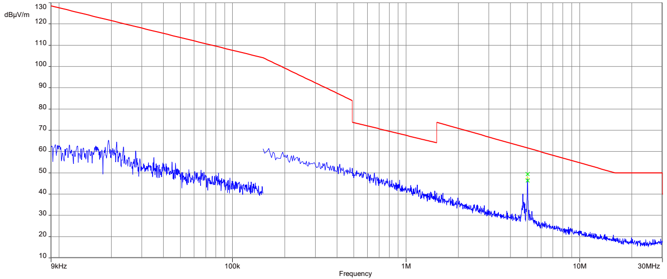
Plot 1: 9 kHz to 30 MHz, low channel, transmit mode
