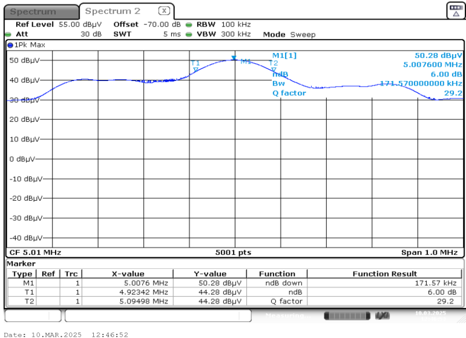
Plot 2: 6dB emission bandwidth
