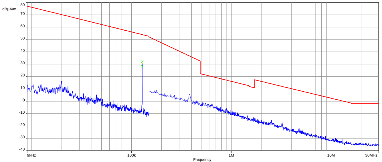
Plot 1: 9 kHz – 30 MHz, magnetic spurious emissions IC
