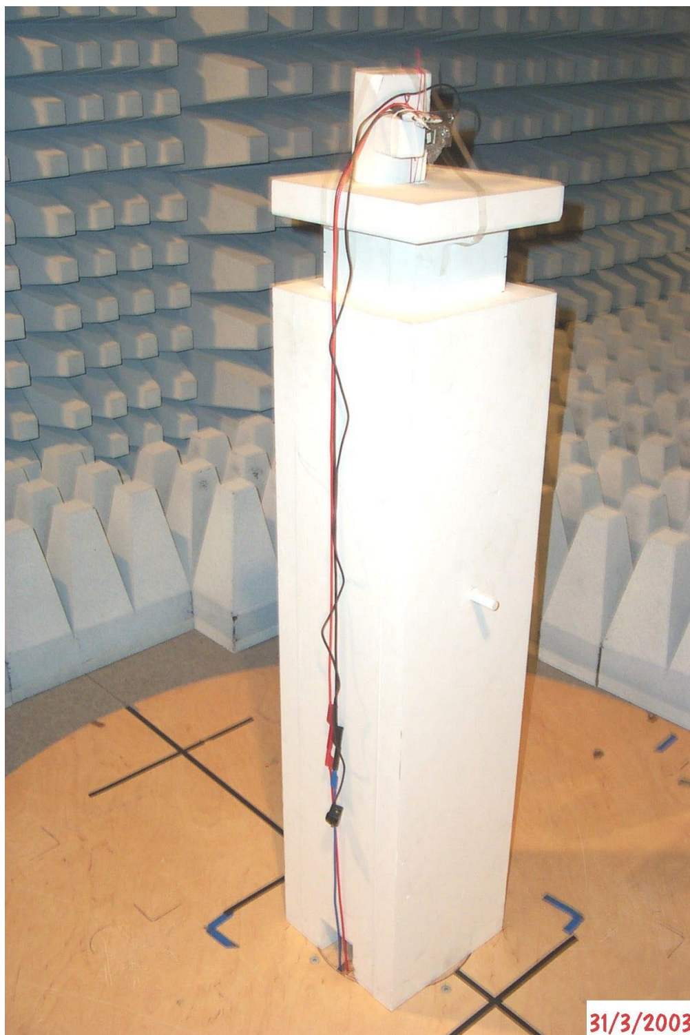
30141_e.jpg BCM001 test set-up emission measurement above 1 GHz
