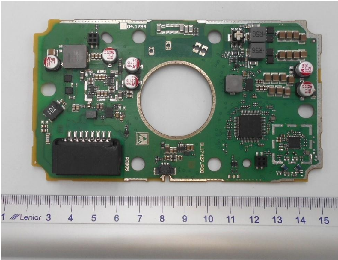
Photo 2 - Main PCB TOP (no shielding)
