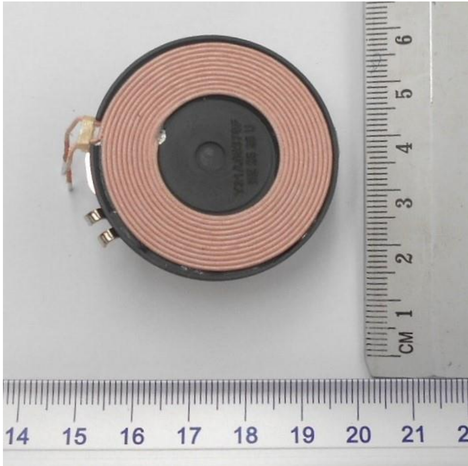
Photo 5 – WPT Coil TOP
