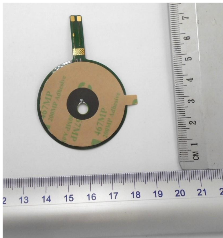
Photo 4 - NFC PCB Flex
