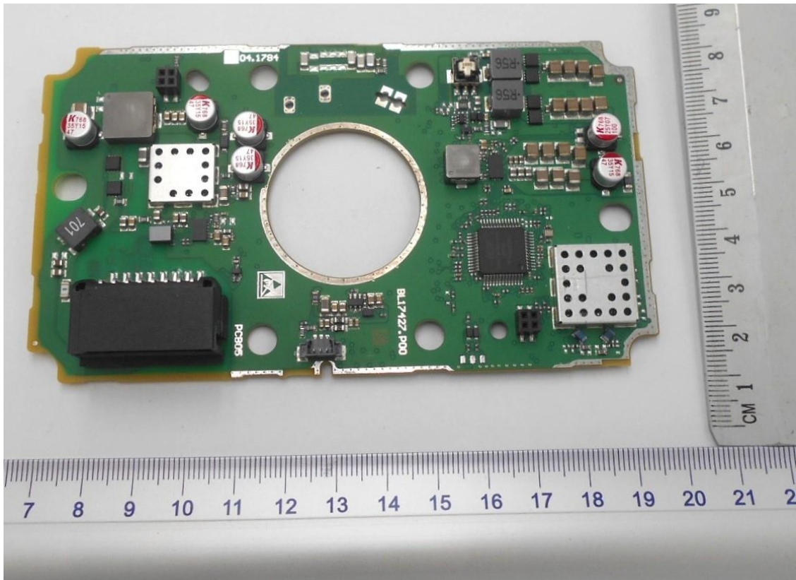
Photo 1 - Main PCB TOP
