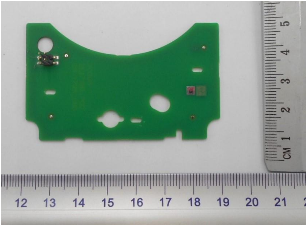
Photo 5 - NFC PCB TOP
