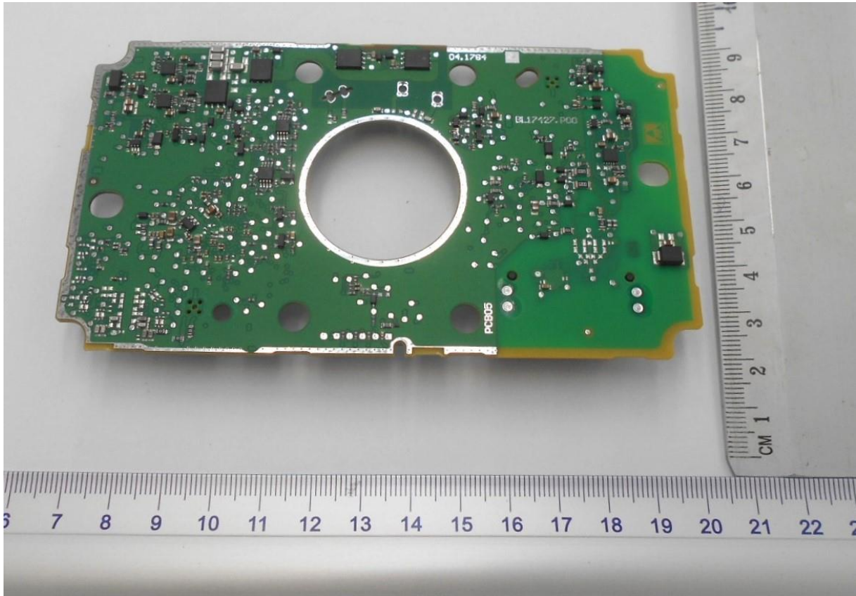
Photo 3 - Main PCB BOTTOM
