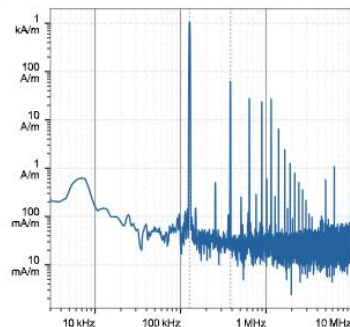
H-field magnitude [RMS] at center location
