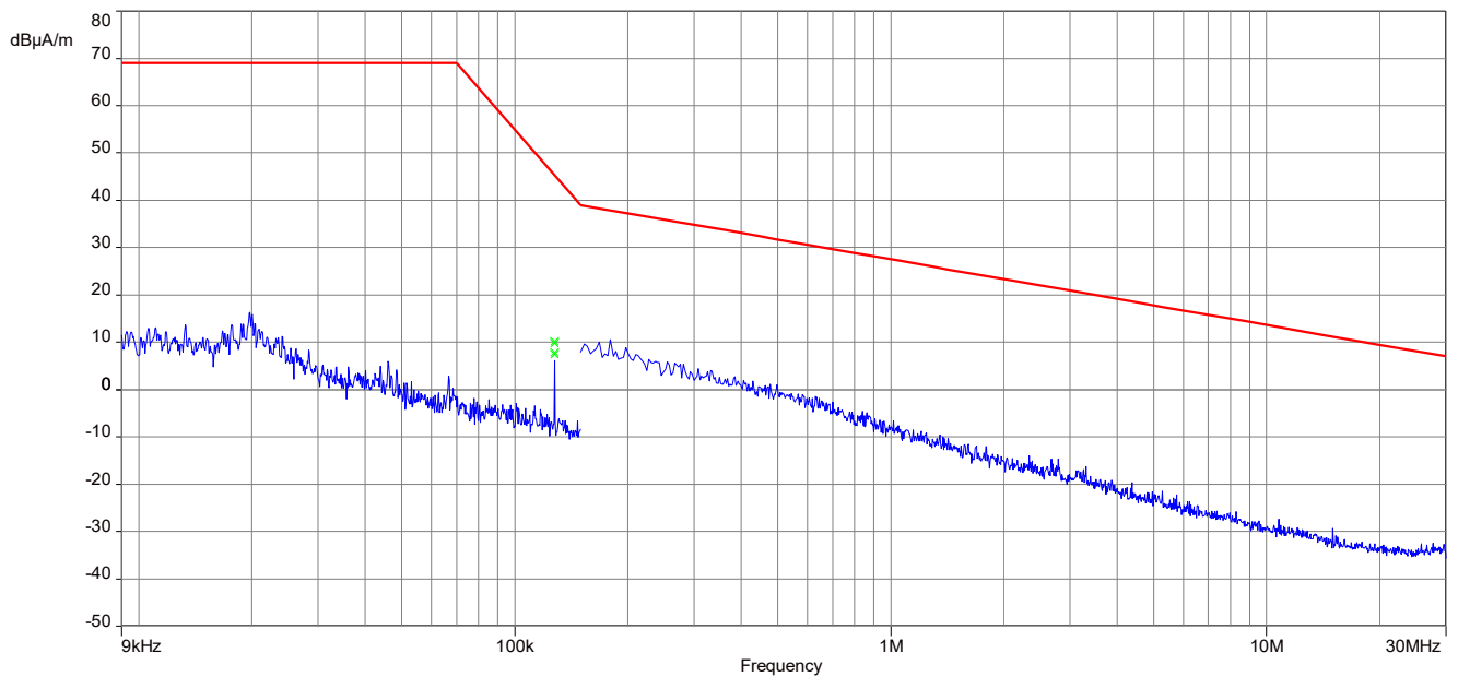
Plot 2: 9 kHz – 30 MHz, magnetic spurious emissions IC, 126 kHz
