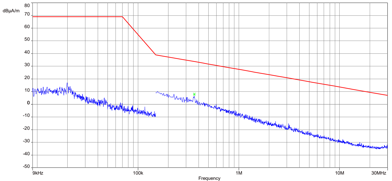
Plot 4: 9 kHz – 30 MHz, magnetic spurious emissions IC, 360 kHz
