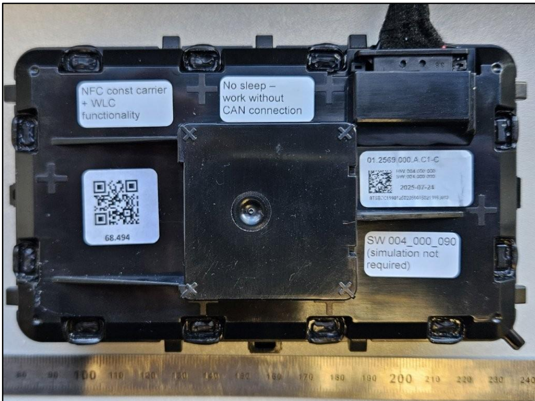
Photo 4: EUT Bottom View
