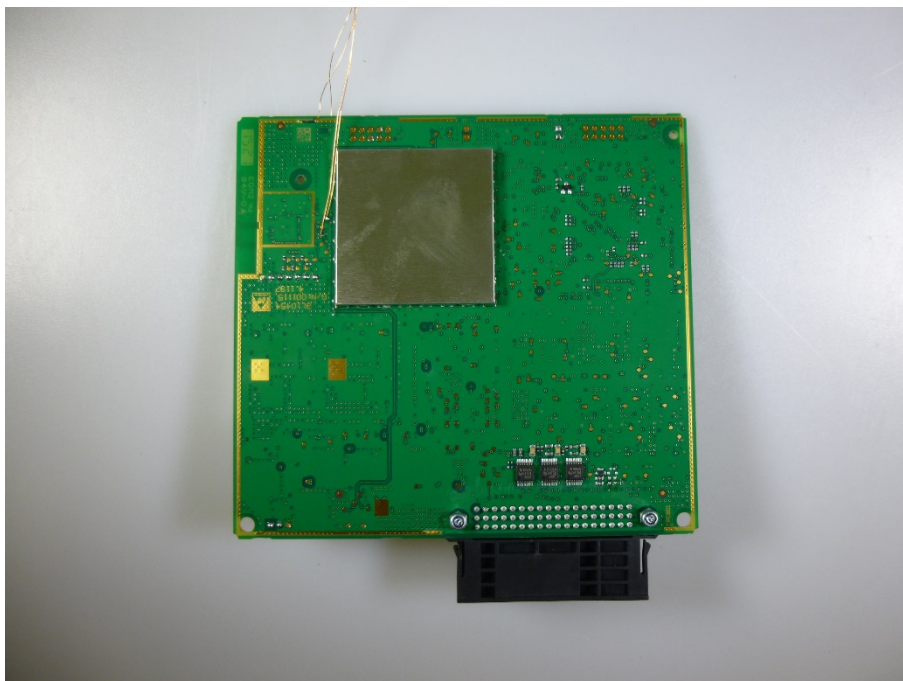
Photo 2: PCB front with shielding
