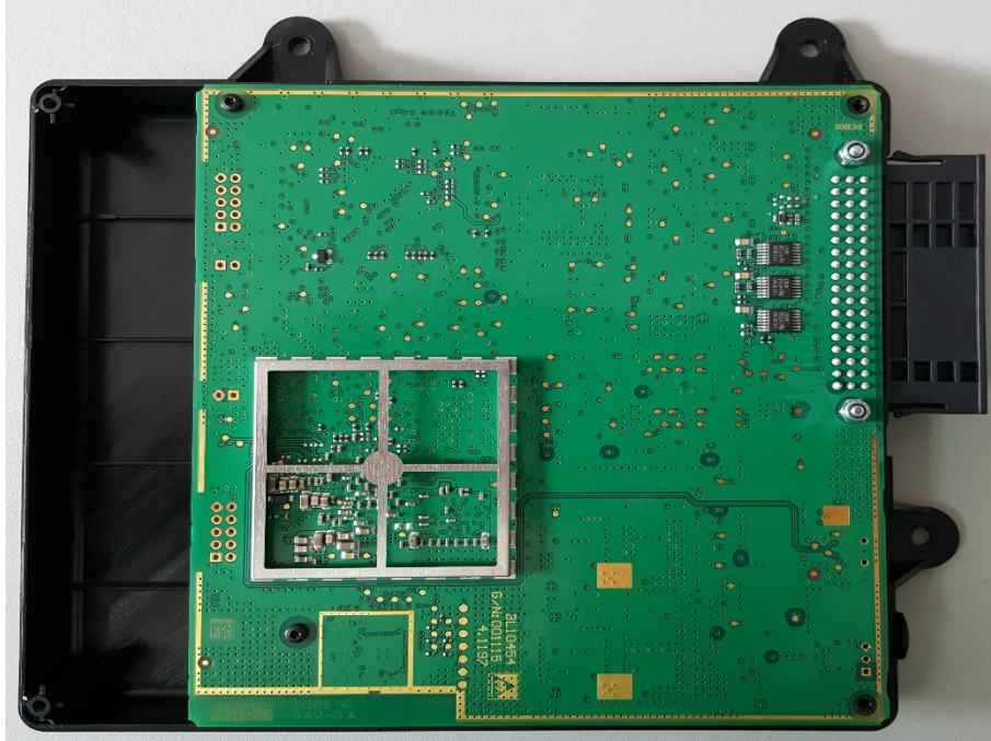
Photo 5: PCB front without shielding (provided by manufacturer)
