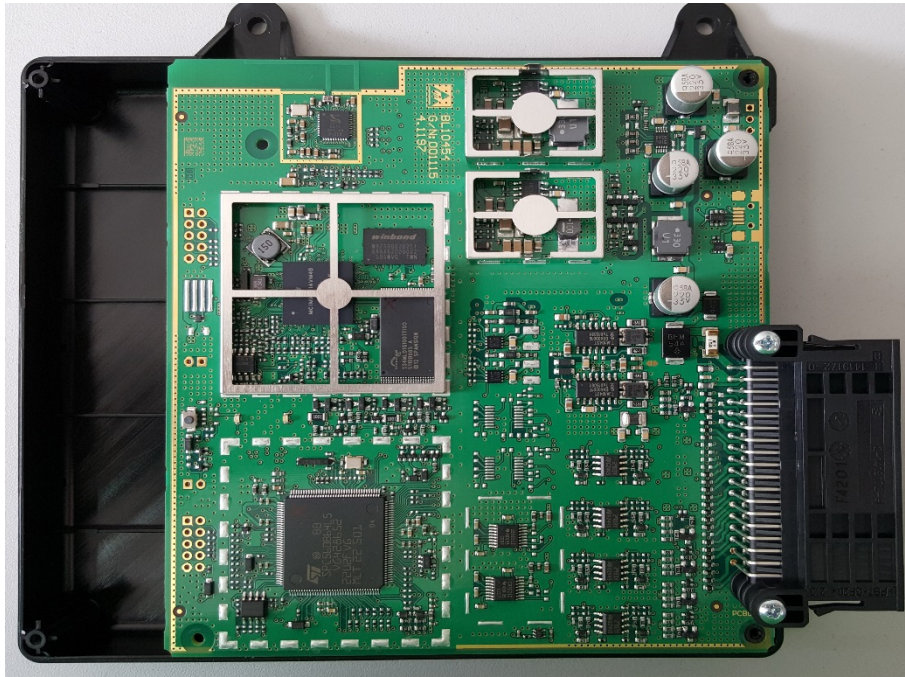
Photo 6: PCB back without shielding (provided by manufacturer)
