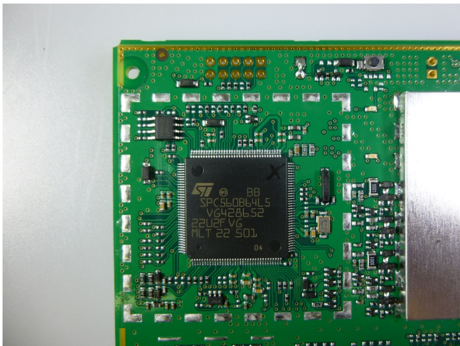
Photo 4: PCB
