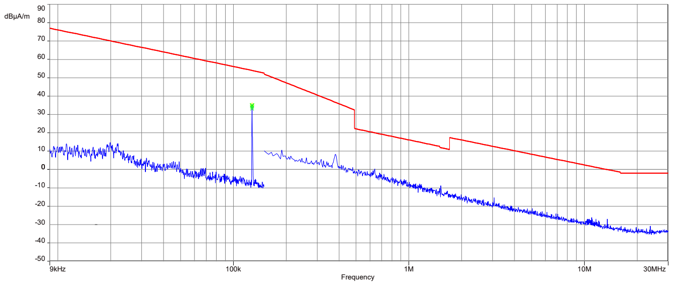
Plot 1: 9 kHz – 30 MHz, magnetic spurious emissions IC
