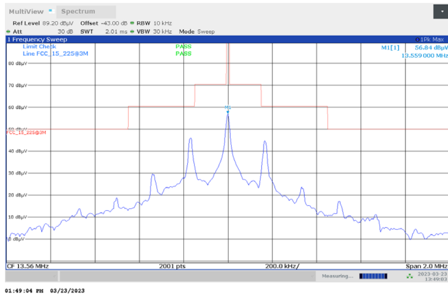
Plot 3: Spectrum mask (the limits are recalculated according to the ANSI C63.10-2013 sub clause 6.4)
