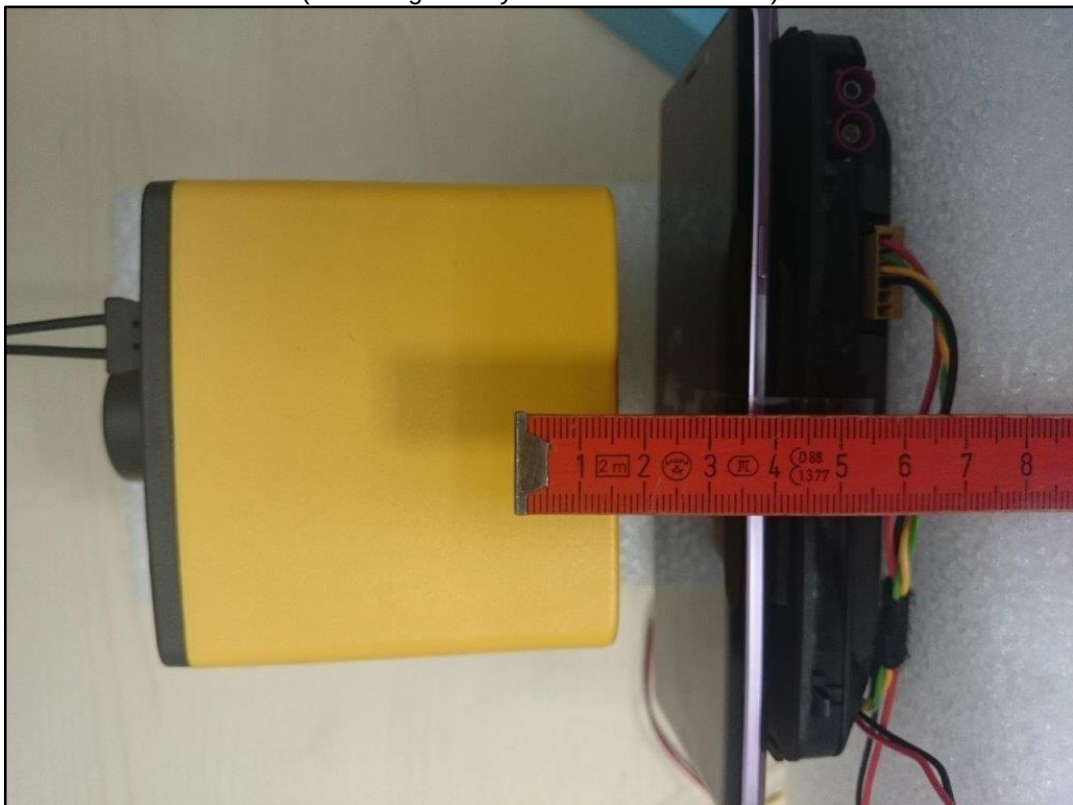
Photo 18: Test position – top side – Wireless charging with EHP50F probe (Samsung Galaxy Note9 / 5cm distance)
