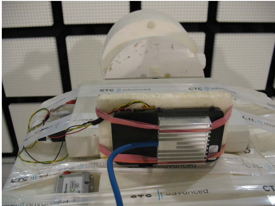
Photo 9: WPC measurements
