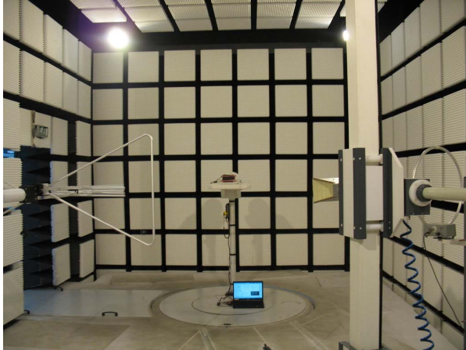
Photo 8: RFID measurements
