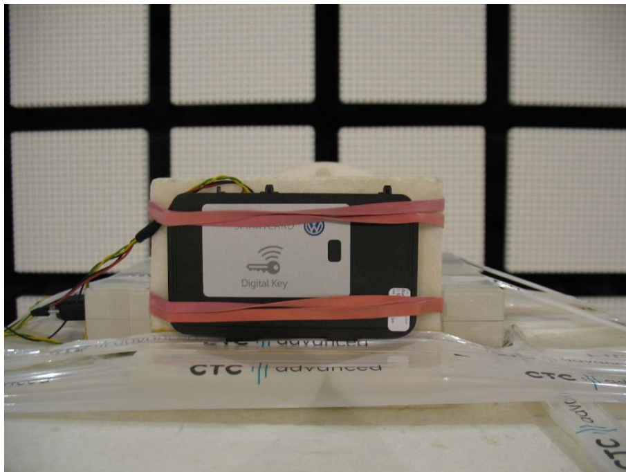
Photo 8: RFID measurements
