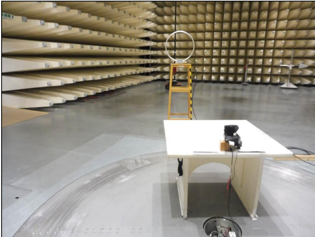
Photo 5: radiated emission 9KHz-30MHz x-axis set 2
