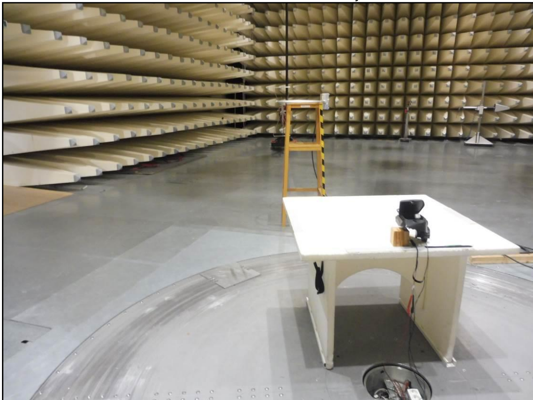
Photo 6: radiated emission 9KHz-30MHz y-axis set 2
