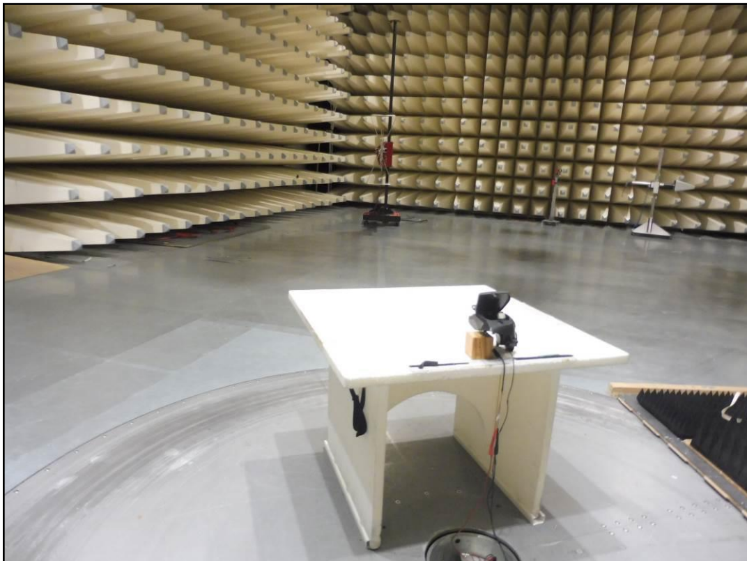
Photo 8: radiated emission 30MHz - 1GHz set 2
