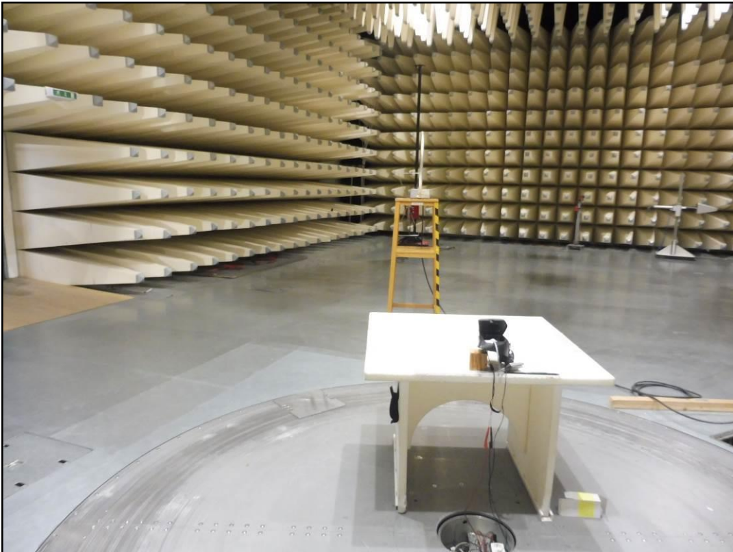
Photo 3: radiated emission 9KHz-30MHz set 1 z-axis
