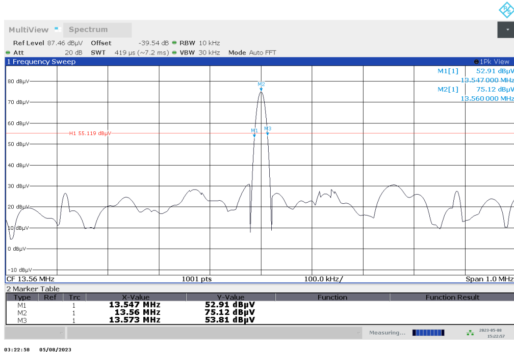
Plot No. 17: 20 dB bandwidth, EUT A
