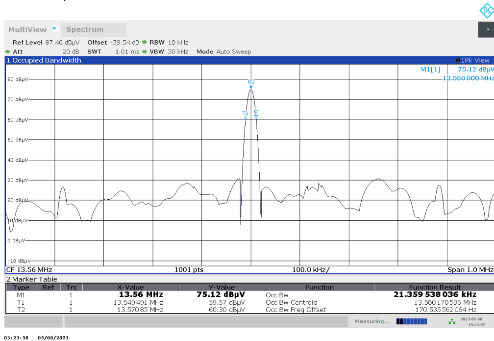
Plot No. 16: 99% Occupied bandwidth, EUT A
