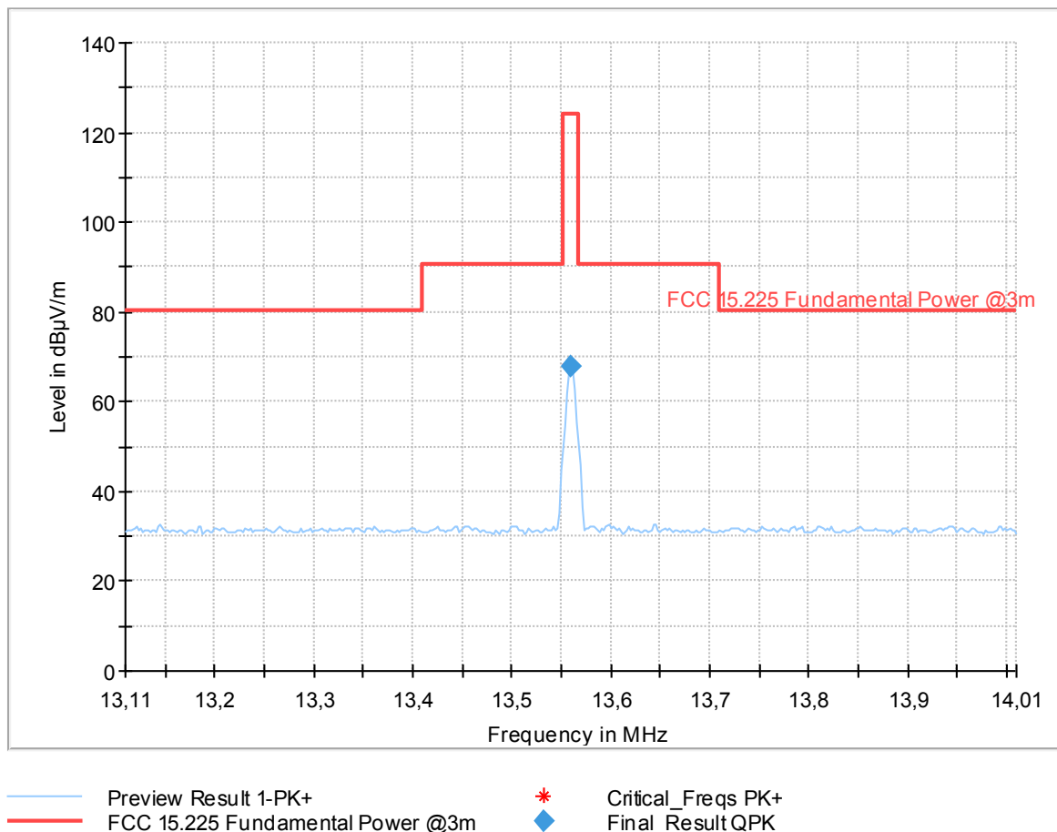
Plot no. 1: Transmitter Spectrum Mask (TSM), lying
