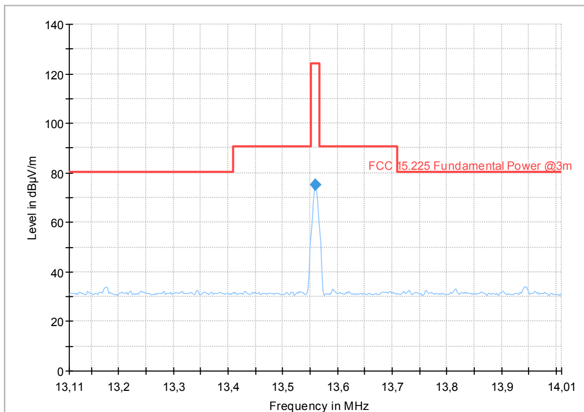
Plot no. 2: Transmitter Spectrum Mask (TSM), staying
