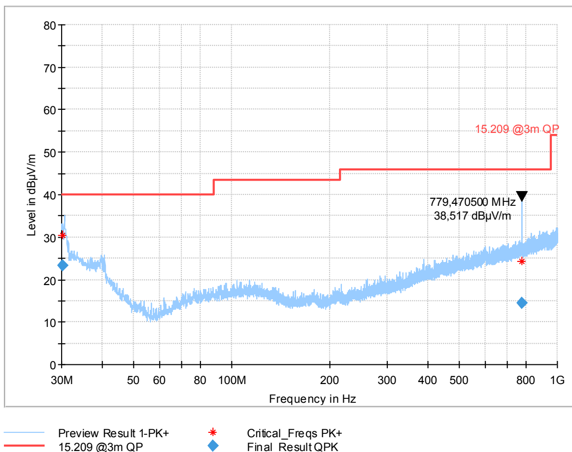
Plot no. 5: Radiated emissions 30 MHz – 1 GHz, hor./vert. polarization, EUT lying
