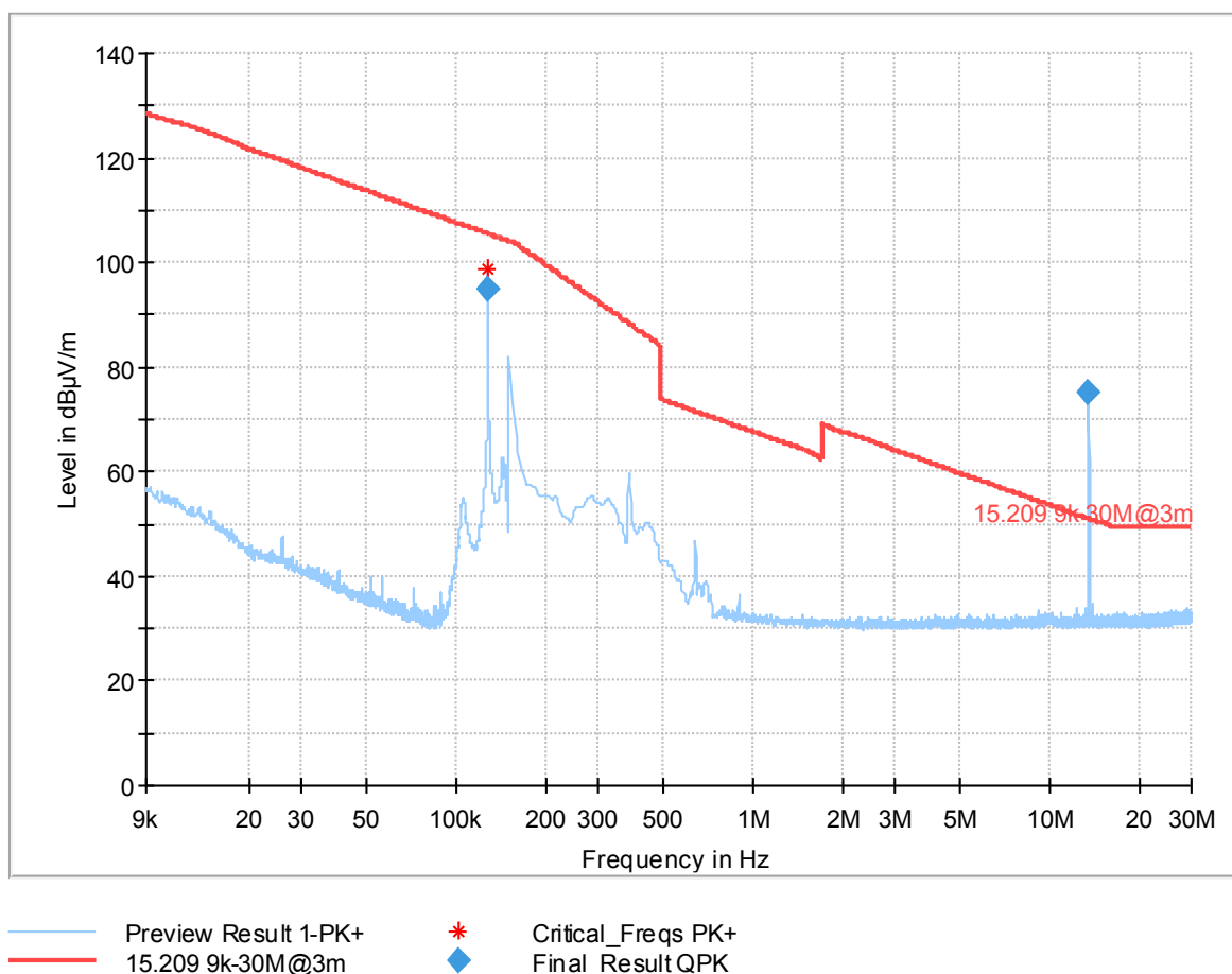
Plot no. 4: Radiated emissions 9 kHz – 30 MHz, EUT staying
