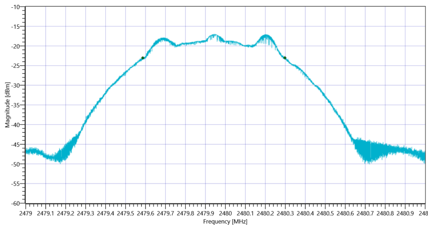
Plot_FCC Part 15.247 Maximum Peak Conducted Output Power DTS ~ BT LE 1 Msps DTS BW_18082021_121958.png
