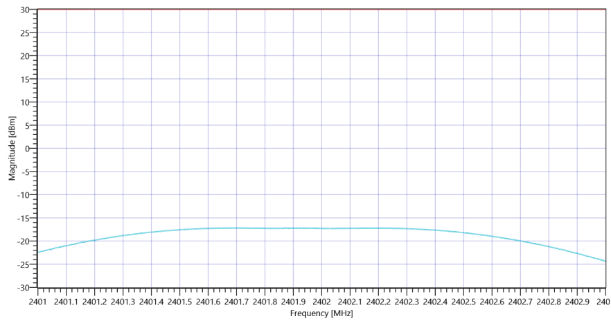
Plot_FCC Part 15.247 Maximum Peak Conducted Output Power DTS ~ BT LE 1 Msp_18082021_121844.png
