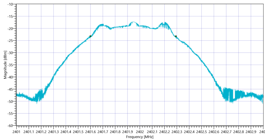
Plot_FCC Part 15.247 Maximum Peak Conducted Output Power DTS ~ BT LE 1 Msps DTS BW_18082021_121826.png
