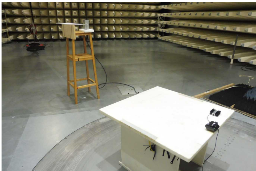
Photo 4: radiated emission with loop antenna, z-axis
