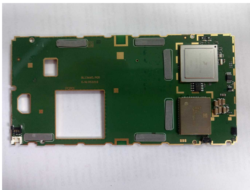
PCB of the EUT (rear view)
