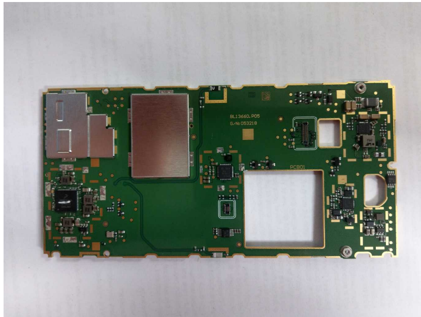
PCB of the EUT (front view)
