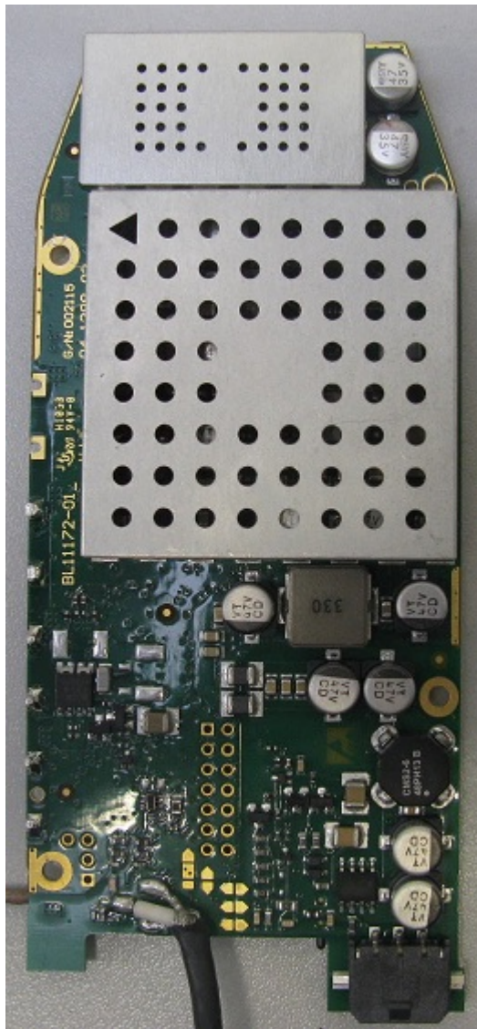
Photo 1: main board frond side
