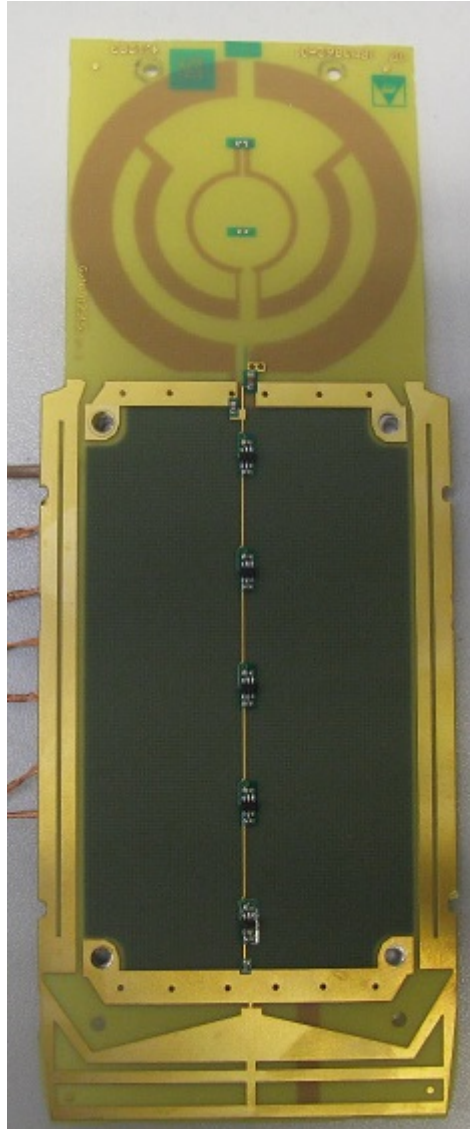
Photo 4: Antenna board front side
