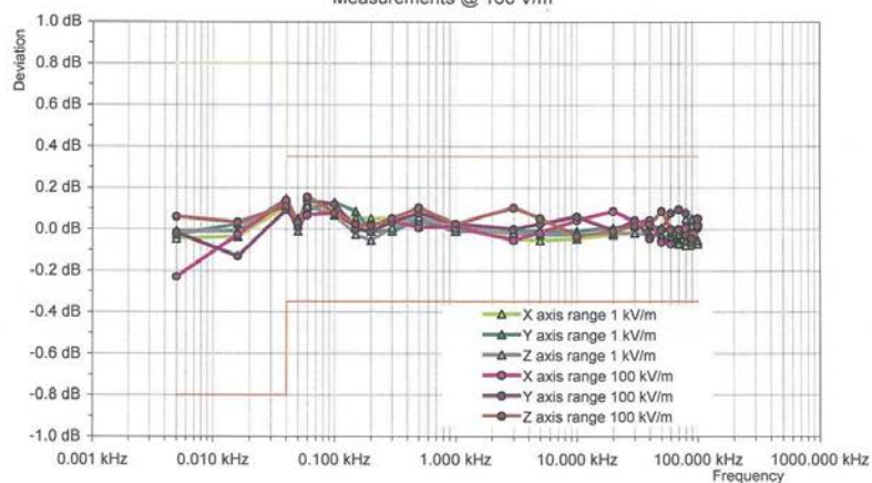
Frequency response EHP50D Electric field
