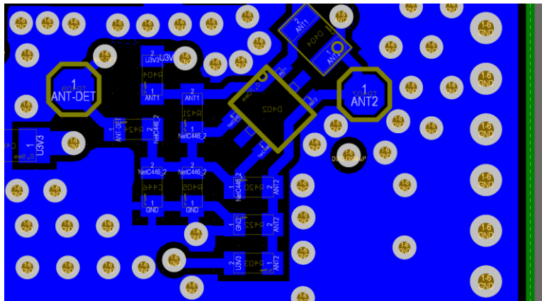
Old PCB
