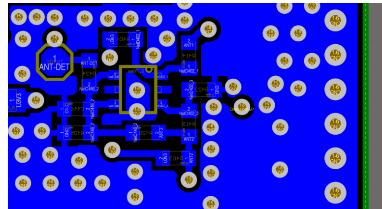
New PCB
