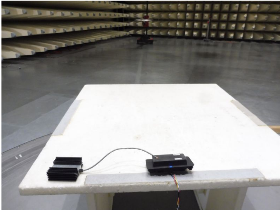
Photo 1: radiated emission < 1GHz
