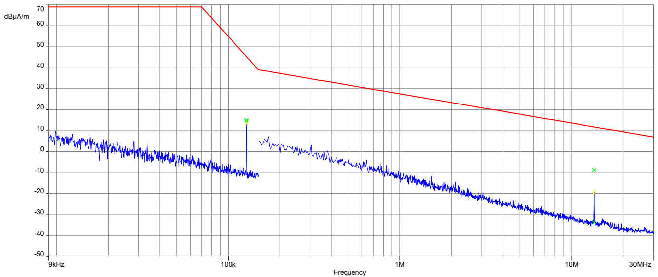
Plot 2: 9 kHz – 30 MHz, magnetic emissions ISCED, 128 kHz single load mode
