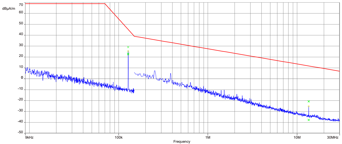
Plot 4: 9 kHz – 30 MHz, magnetic emissions ISCED, 128 kHz dual load mode
