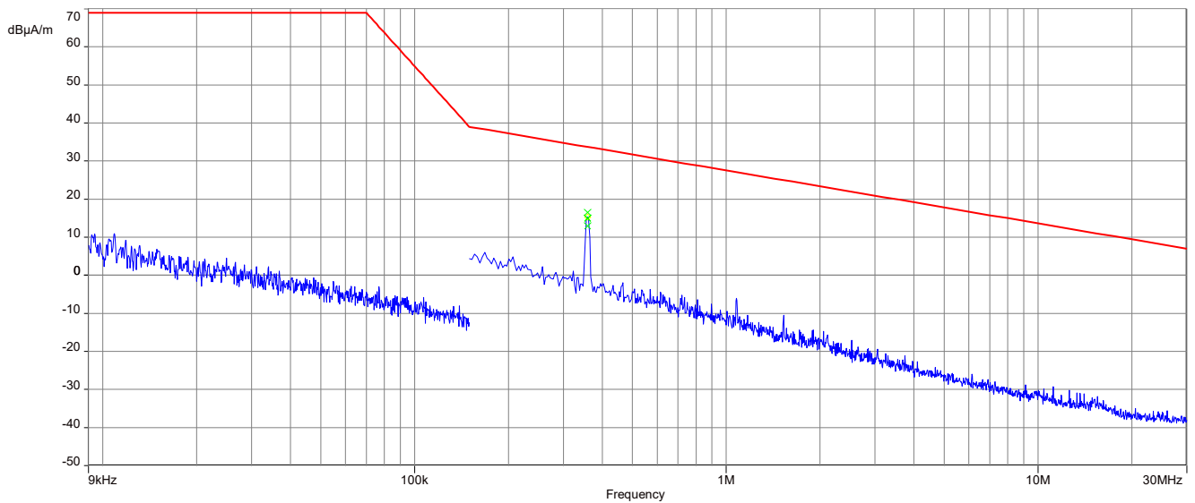
Plot 2: 9 kHz – 30 MHz, magnetic emissions ISSED, 360 kHz single load mode
