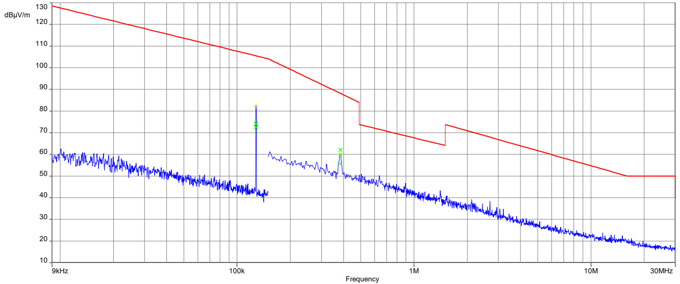
Plot 3: 9 kHz – 30 MHz, magnetic emissions FCC, 128 kHz dual load mode
