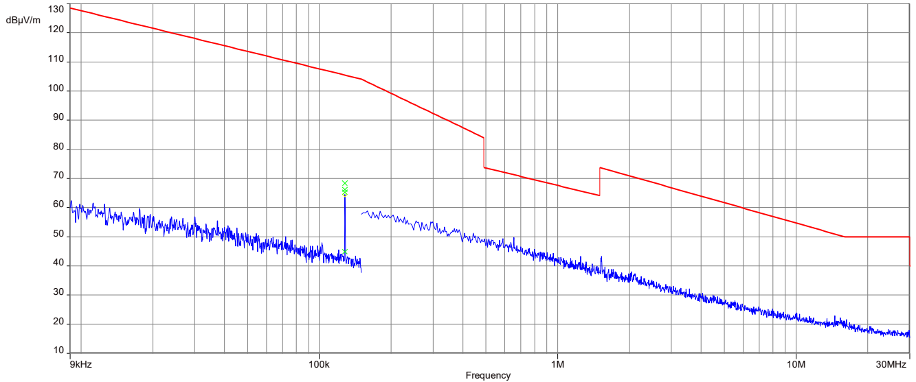
Plot 1: 9 kHz – 30 MHz, magnetic emissions FCC, 128 kHz single load mode
