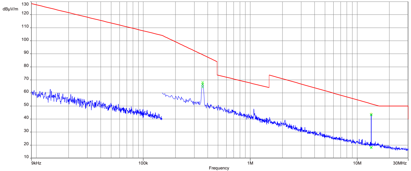
Plot 1: 9 kHz – 30 MHz, magnetic emissions FCC, 360 kHz single load mode
