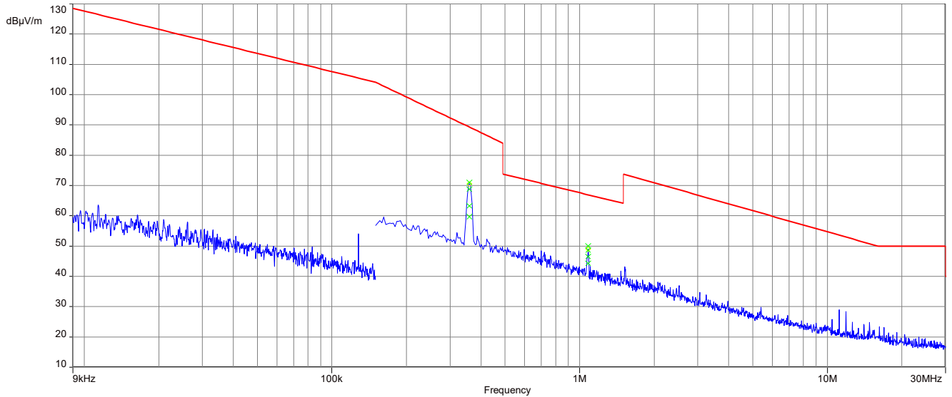
Plot 3: 9 kHz – 30 MHz, magnetic emissions FCC, 360 kHz dual load mode
