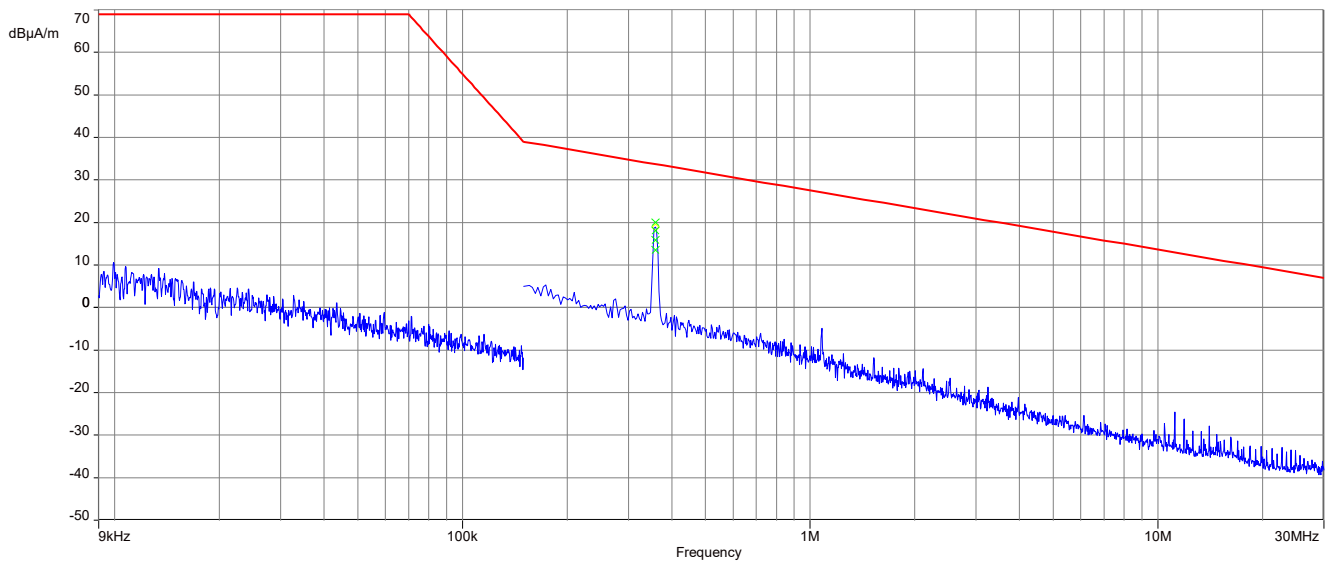
Plot 4: 9 kHz – 30 MHz, magnetic emissions ISCED, 360 kHz dual load mode
