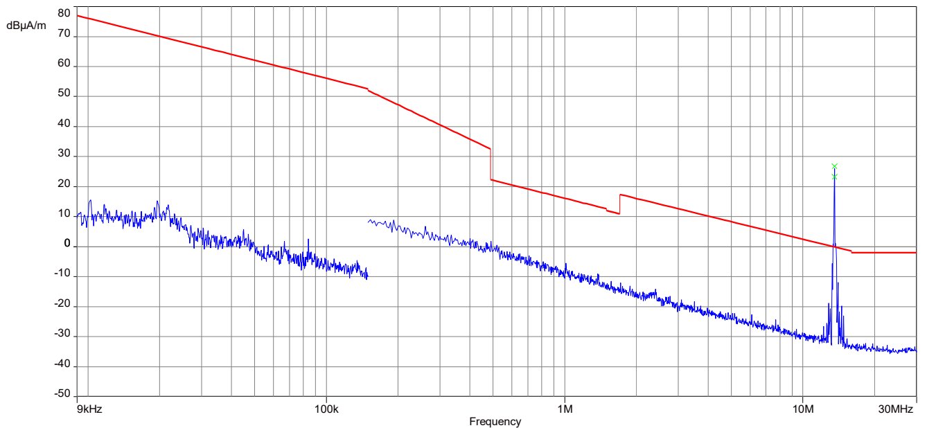
Plot 2: 9 kHz – 30 MHz, magnetic emissions ISCED
