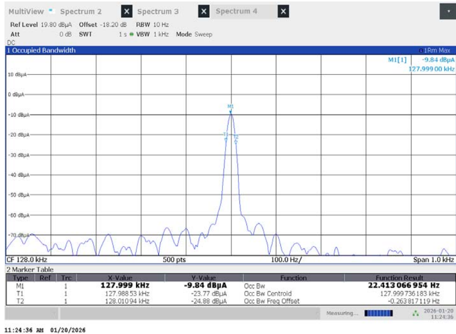
Plot 1: 99 % emission bandwidth, 128 kHz
