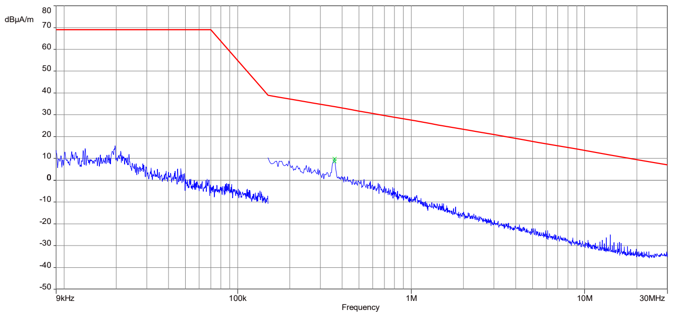
Plot 4: 9 kHz – 30 MHz, magnetic spurious emissions ISED, 360 kHz
