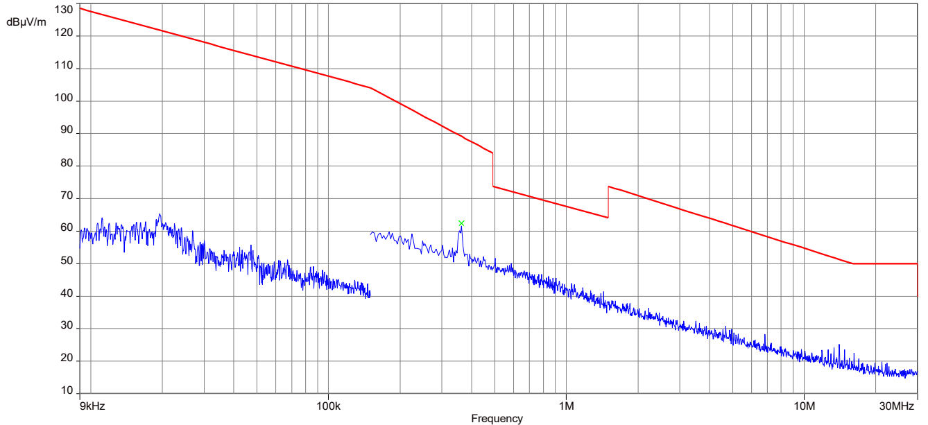
Plot 3: 9 kHz – 30 MHz, magnetic spurious emissions FCC, 360 kHz
