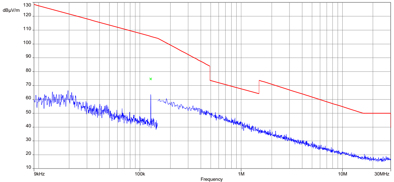
Plot 1: 9 kHz – 30 MHz, magnetic spurious emissions FCC, 126 kHz
