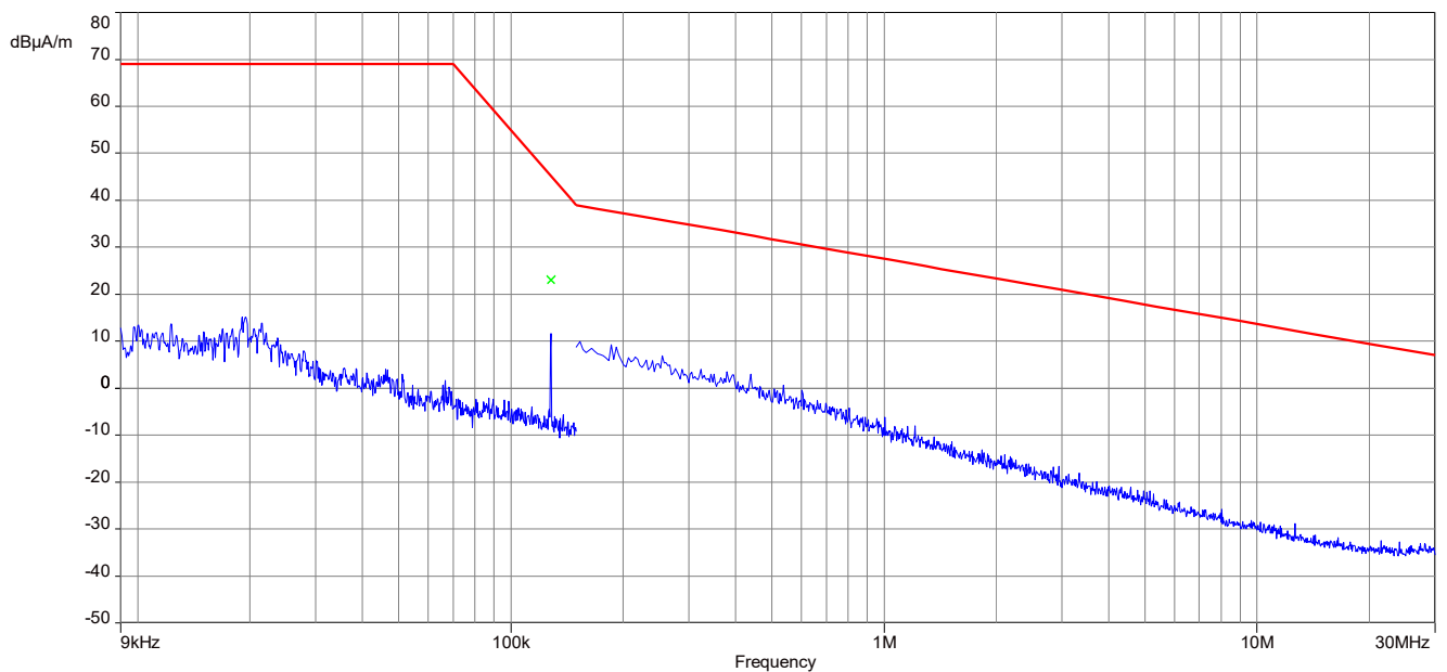
Plot 2: 9 kHz – 30 MHz, magnetic spurious emissions ISSED, 126 kHz
