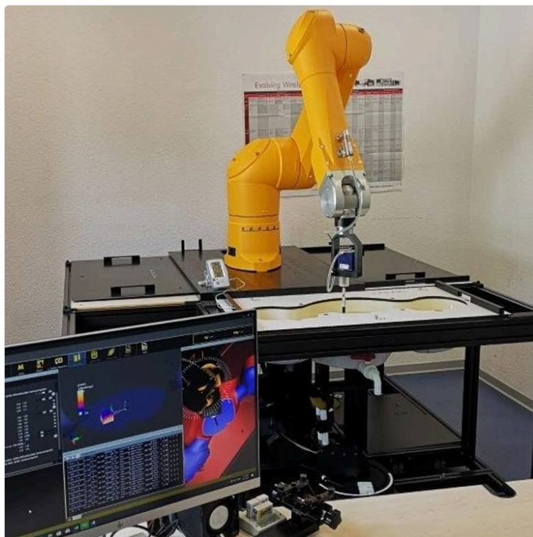
Photo 1 DASY 6/8 Test System
