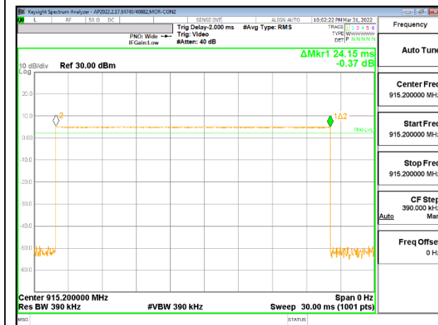
PULSE WIDTH – 50 kbps
