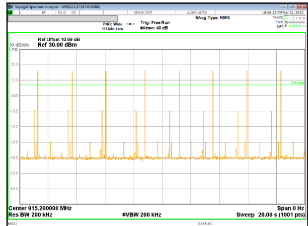
NUMBER OF PULSES IN 20 SECOND OBSERVATION PERIOD – 150 kbps
