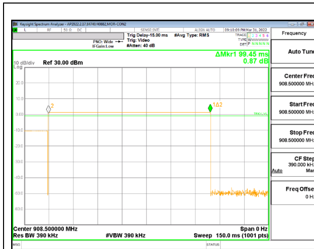
PULSE WIDTH – 35.56 kbps
