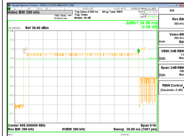
PULSE WIDTH – 200 kbps
