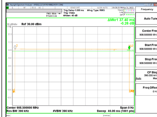
PULSE WIDTH – 142.22 kbps
