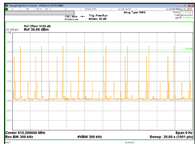
NUMBER OF PULSES IN 10 SECOND OBSERVATION PERIOD – 200 kbps Note: Sweep time is 20s, however with center line being 10s, there are 4 pulses within a 10s observation period.
