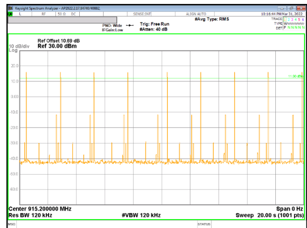
NUMBER OF PULSES IN 20 SECOND OBSERVATION PERIOD – 50 kbps
