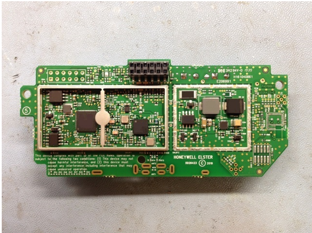
Figure 3: Top View without Shield – Model GNICNZ
