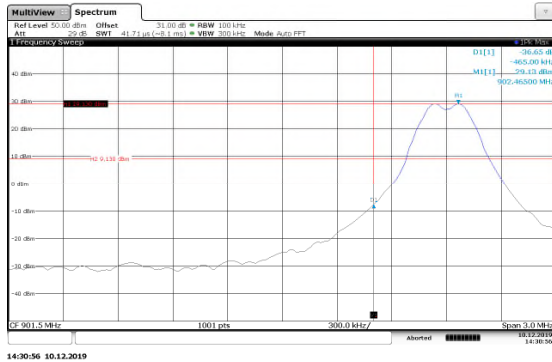
Figure 7.5.1.2-17: Lower Band-edge 150kbps
