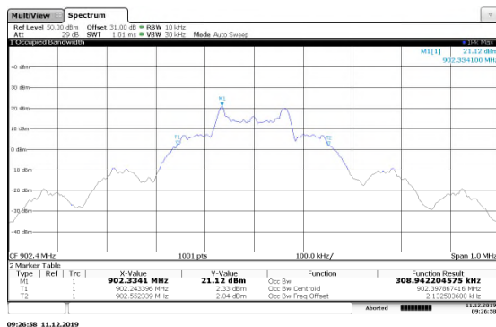
Figure 7.4.4.2-8: 99% OBW Low Channel 142.2kpbs
