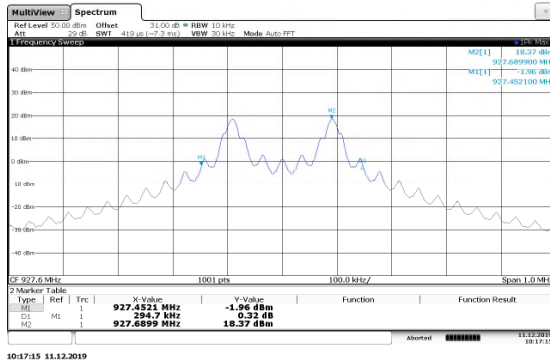
Figure 7.4.4.2-5: 20dB BW High Channel 35.5kpbs
