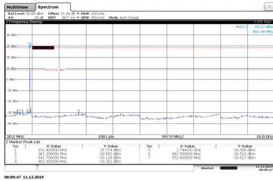
Figure 7.5.2.2-15: 30MHz–10GHz High Channel 200kbps
