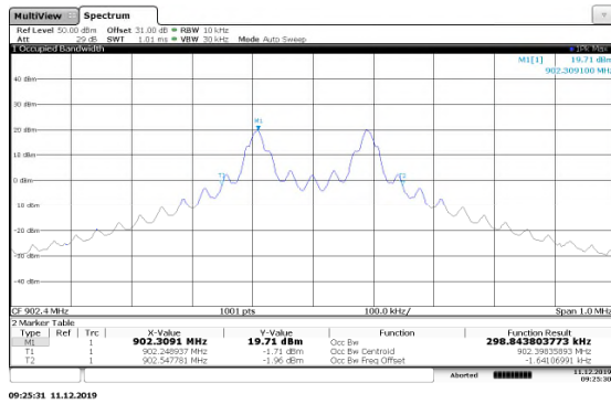
Figure 7.4.4.2-2: 99% OBW Low Channel 35.5kpbs
