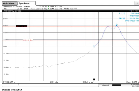
Figure 7.5.1.2-19: Lower Band-edge 200kbps
