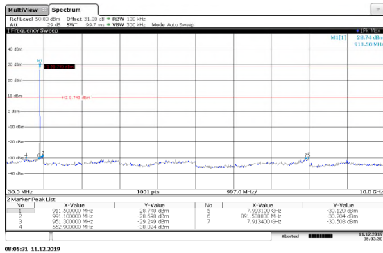
Figure 7.5.2.2-11: 30MHz-10GHz Mid Channel 150kpbs
