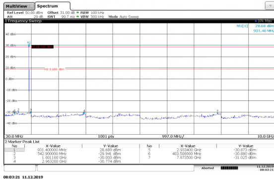
Figure 7.5.2.2-9: 30MHz-10GHz High Channel 50kpbs
