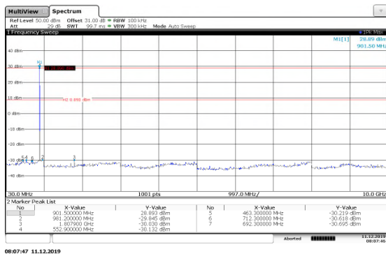
Figure 7.5.2.2-13: 30MHz-10GHz Low Channel 200kpbs
