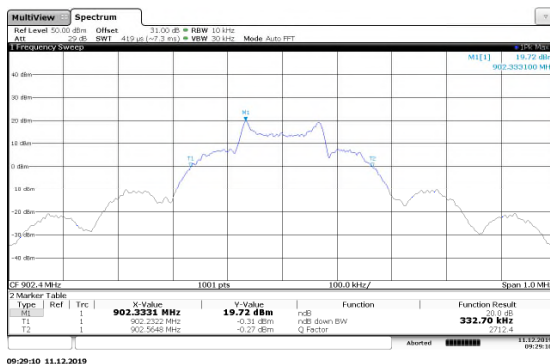
Figure 7.4.4.2-7: 20dB BW Low Channel 142.2kpbs
