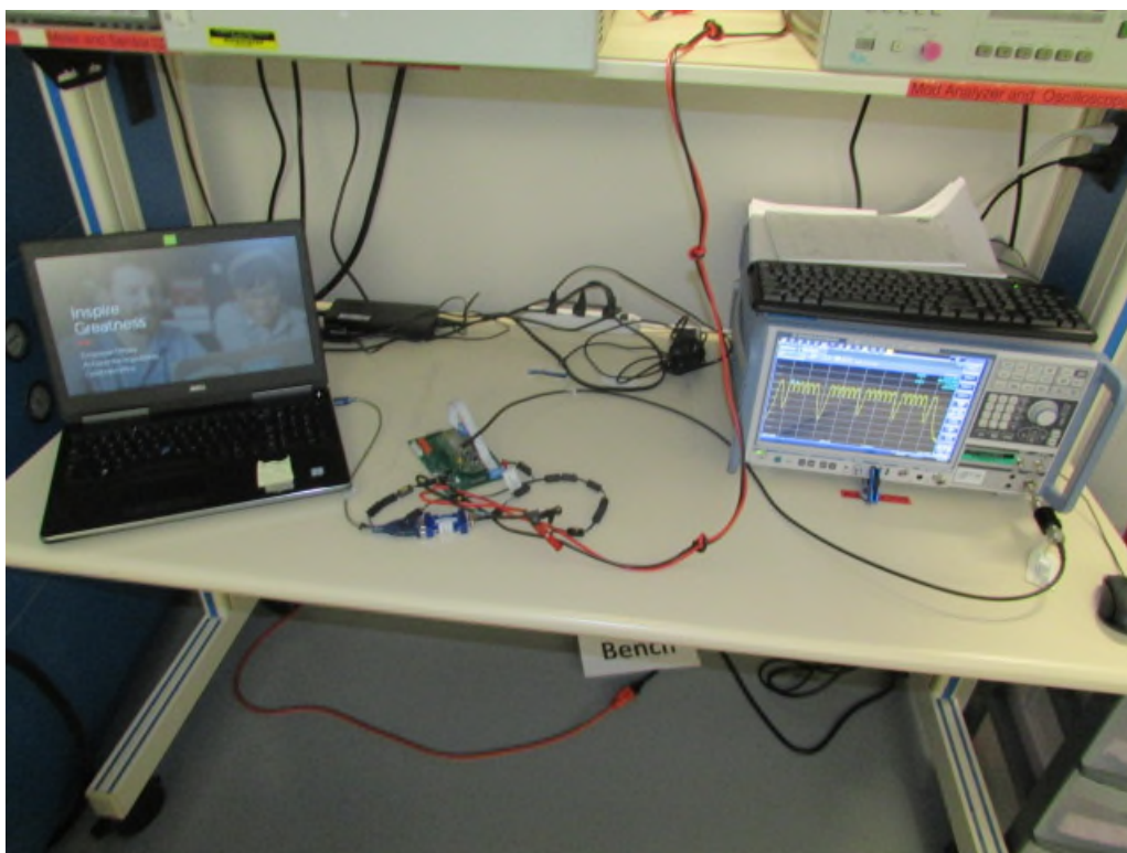
Figure 8: Conducted Emissions
