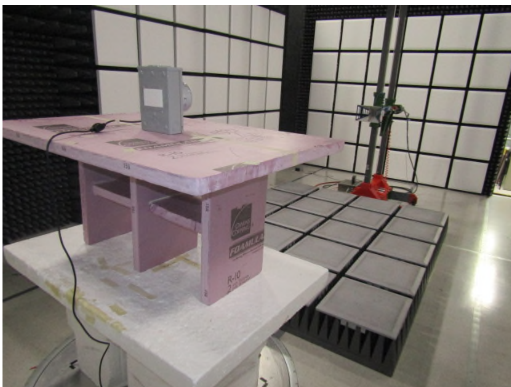
Figure 4: Radiated Emissions – Front – Above 1GHz – ZPOS
