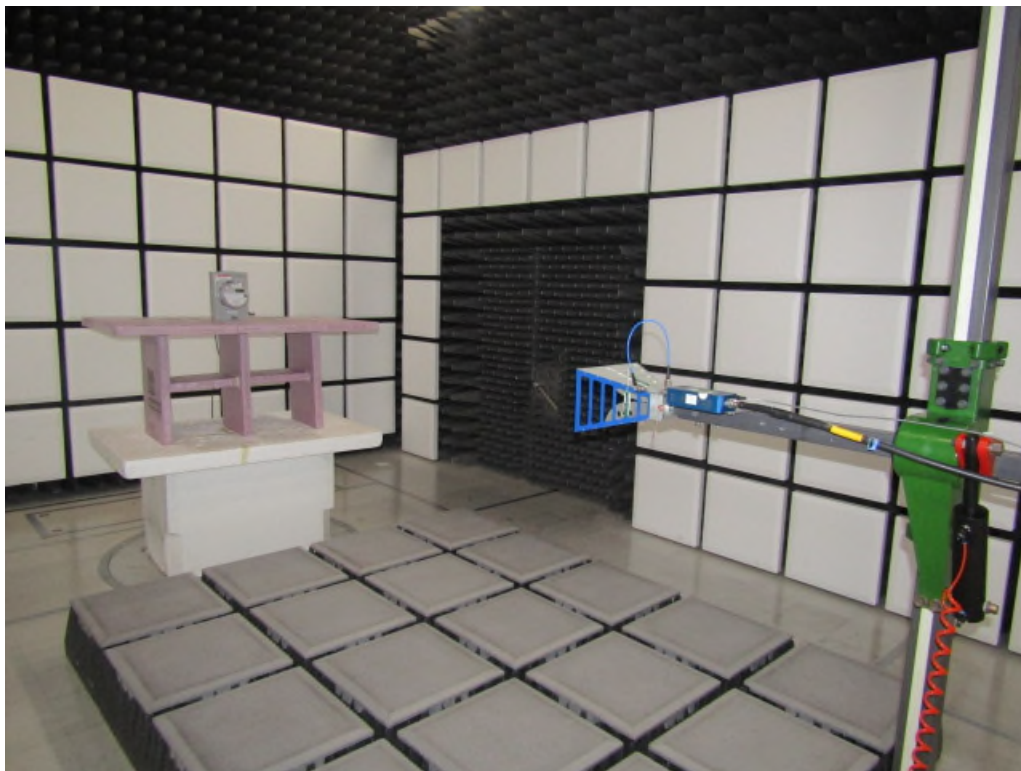
Figure 3: Radiated Emissions – Back – Above 1GHz- YPOS
