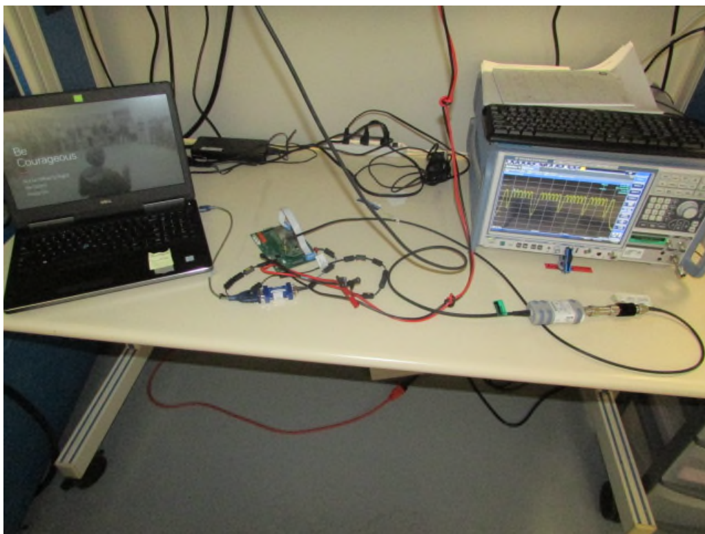
Figure 7: Conducted Emissions
