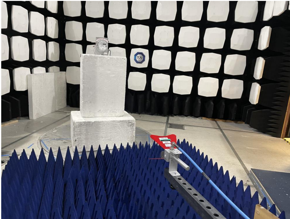
Figure3 – Test Set up - Radiated Emissions <10 GHz
