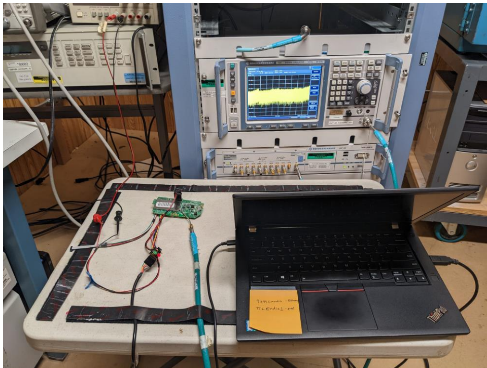
Figure5 – Test Set up – Antenna Port Measurement
