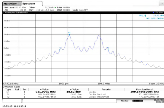
Figure 7.4.4.2-4: 99% OBW Mid Channel 35.5kbps
