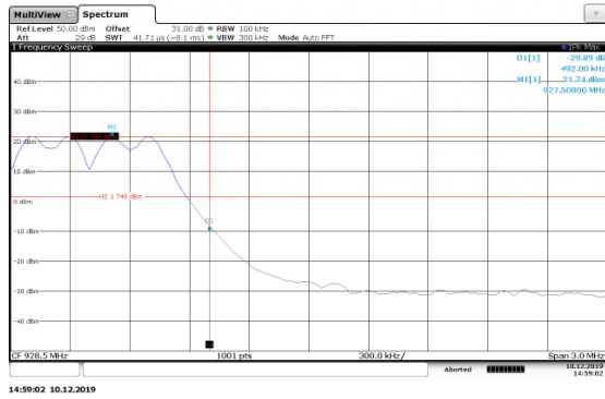
Figure 7.5.1.2-16: Upper Band-edge 200kbps
