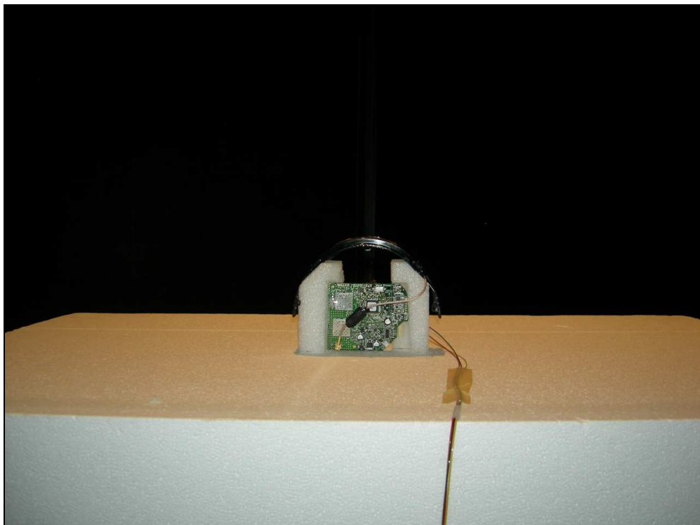
Figure 2: Radiated Emissions – Internal Antenna
