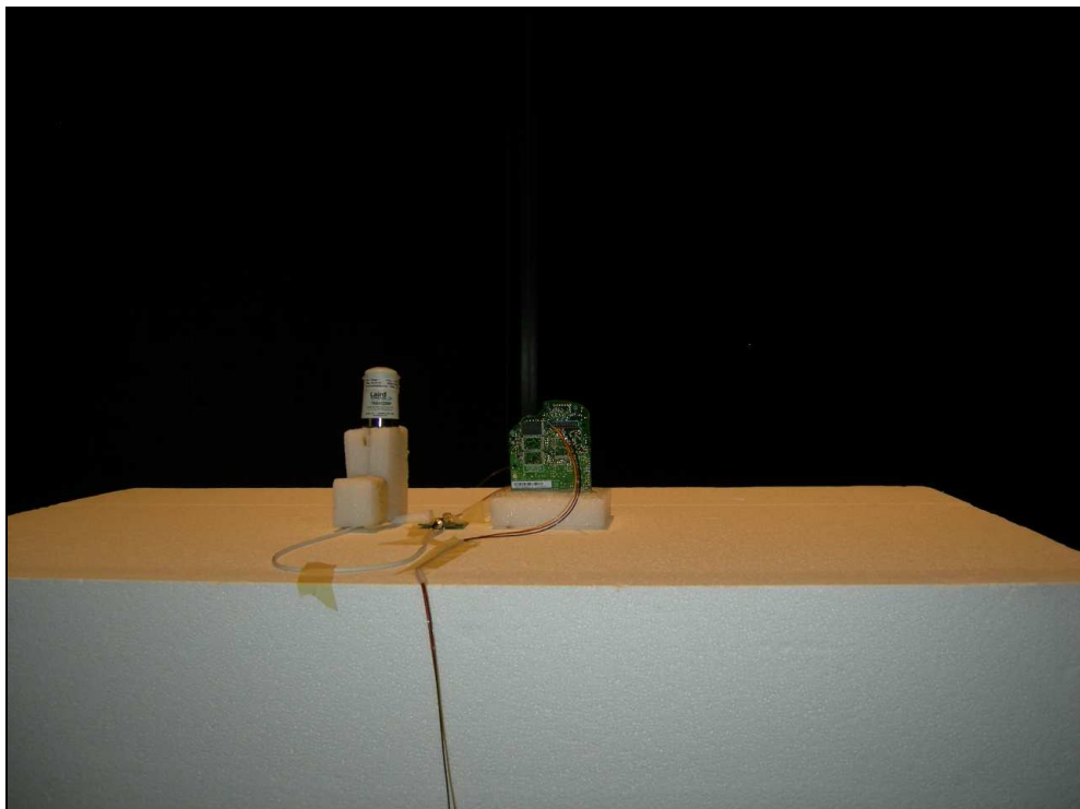
Figure 6: Radiated Emissions – Stubby Antenna
