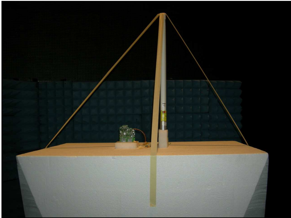
Figure 3: Radiated Emissions – Monopole Antenna
