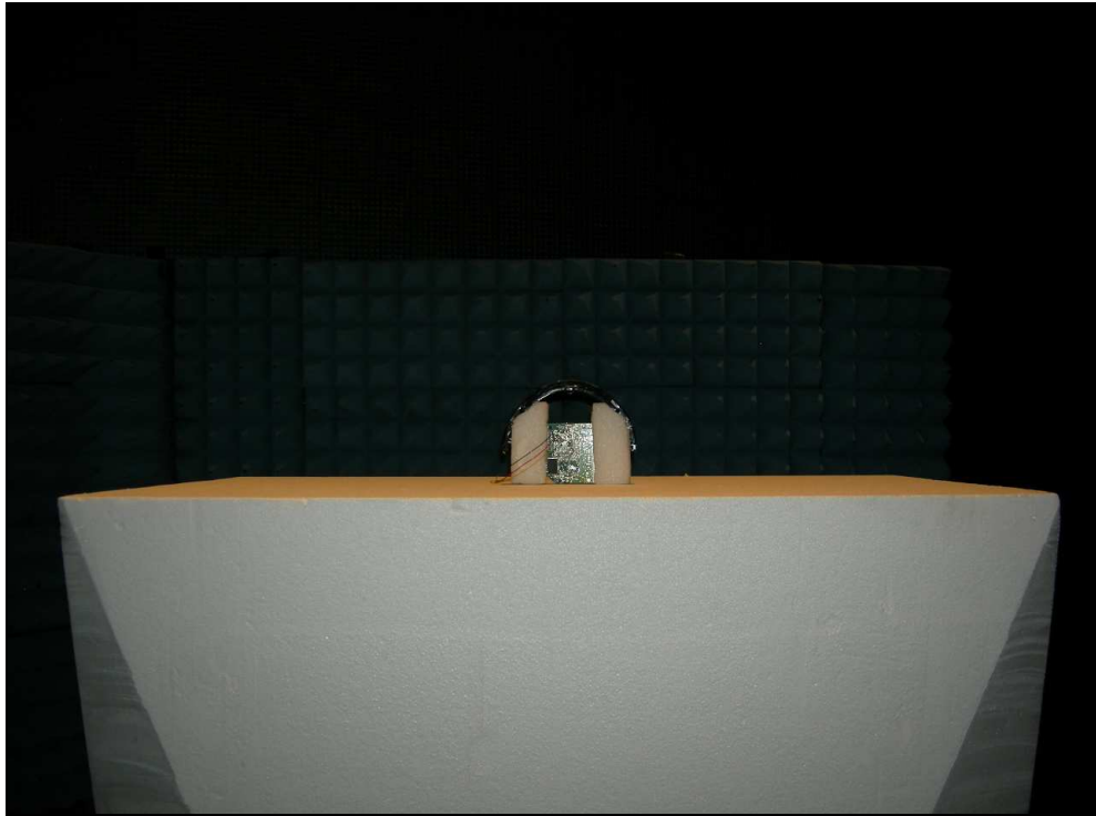
Figure 1: Radiated Emissions – Internal Antenna
