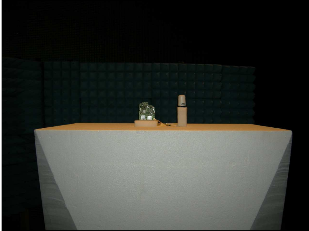
Figure 5: Radiated Emissions – Stubby Antenna
