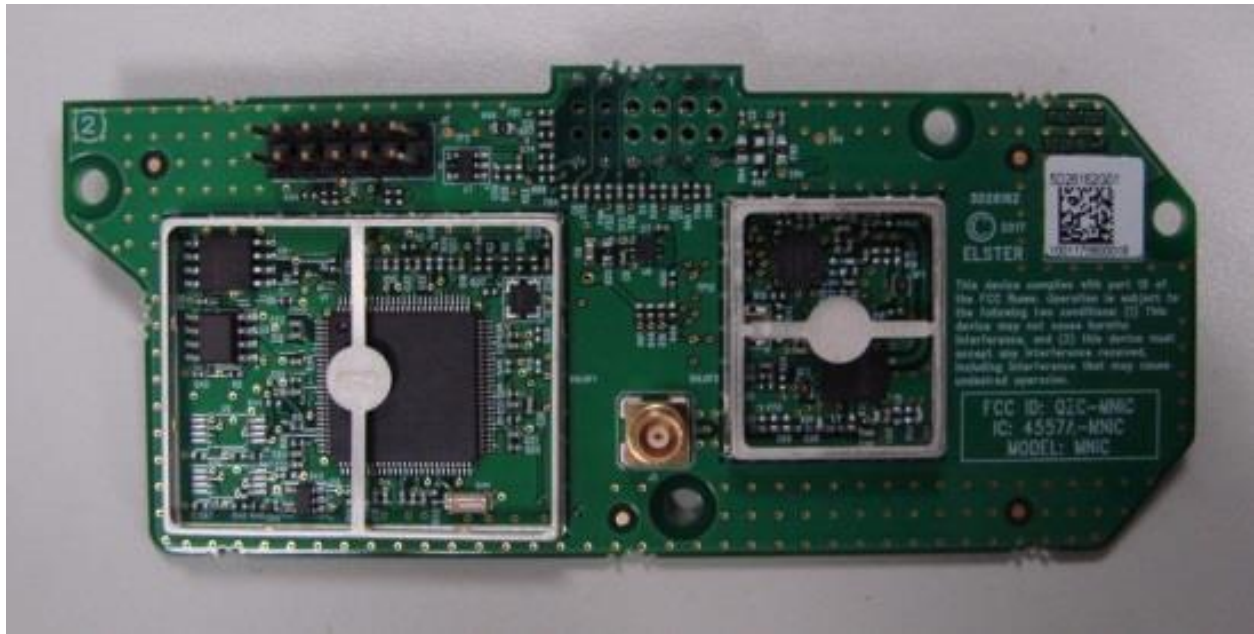
MNIC PCBA top view, shield can lids removed
