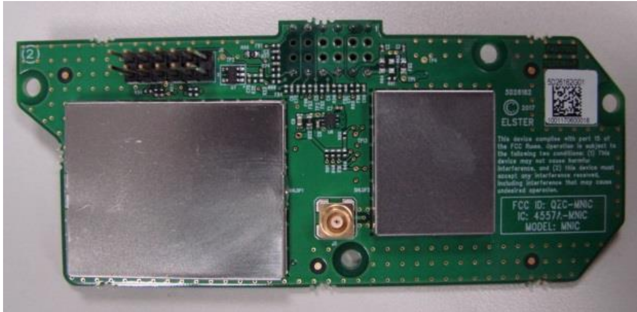
SynergyNet Mini Network Interface Card (MNIC) Printed Circuit Board Assembly (PCBA) top view
