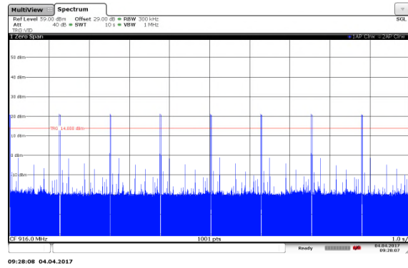
Figure 7.4.3.2-6: Number of Occurrences 200kbps
