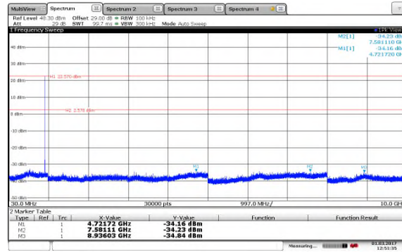
Figure 7.5.2.2-9: 30MHz-10GHz High Channel 200kbps
