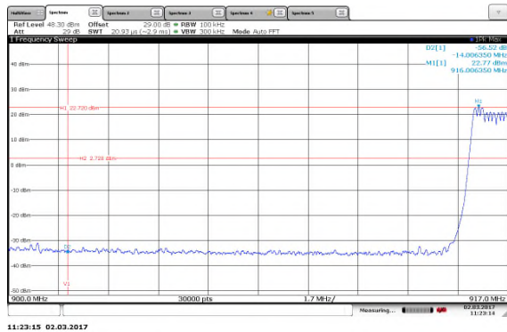
Figure 7.5.1.2-7: Lower Band-edge 35.5kbps
