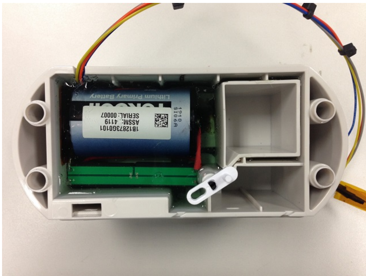
Figure 8: Module Installed and Incased in Epoxy
