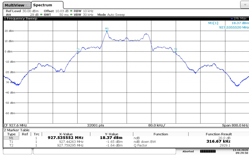
Figure 7.4.4.2-10: 20dB BW High Channel – 142.2kbps
