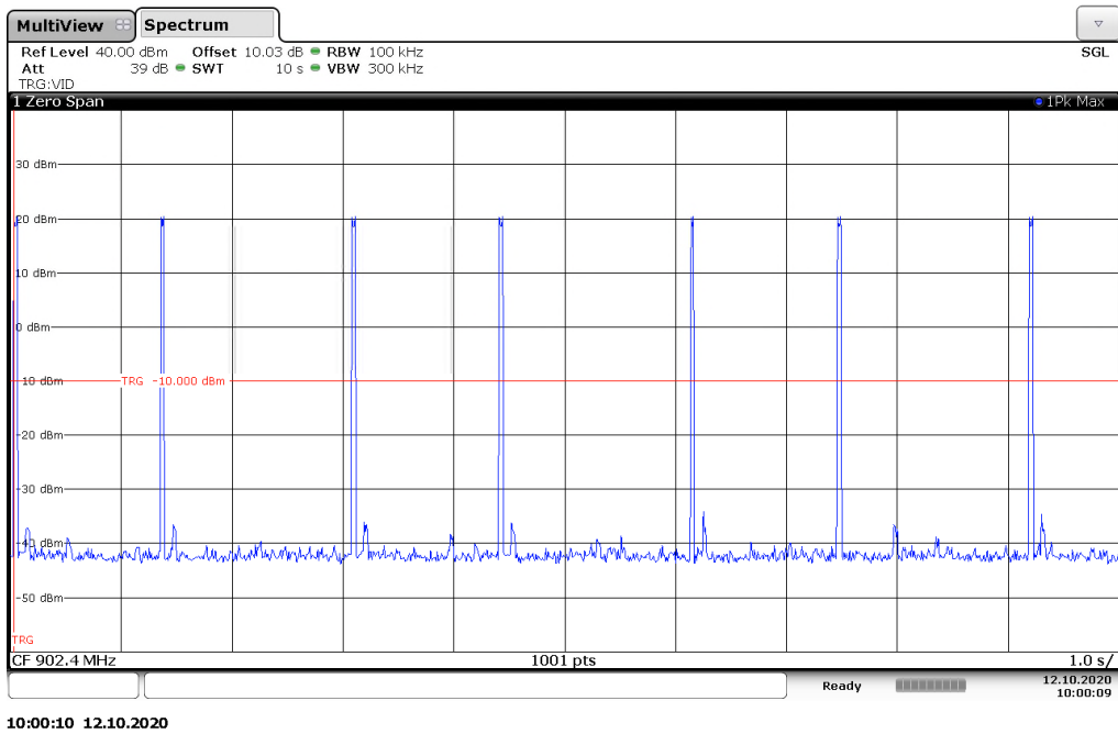
Figure 7.4.3.2-4: Dwell Time – 142.2kbps – Number of Occurrences
