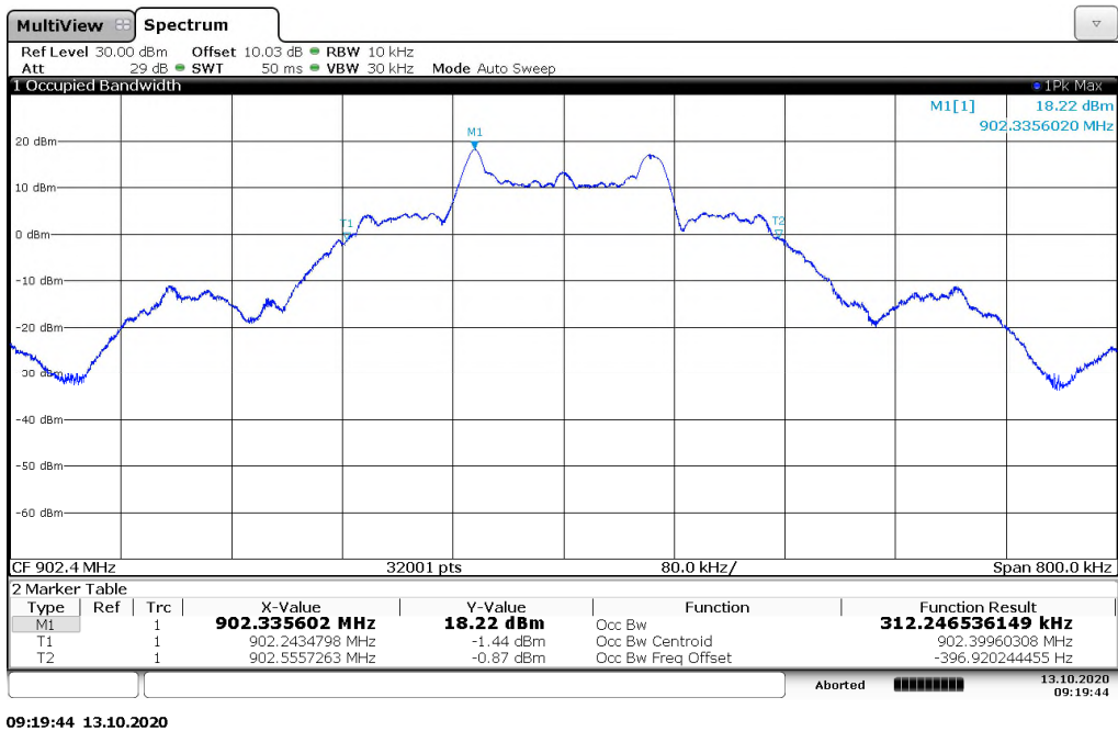
Figure 7.4.4.2-7: 99% OBW Low Channel – 142.2kbps
