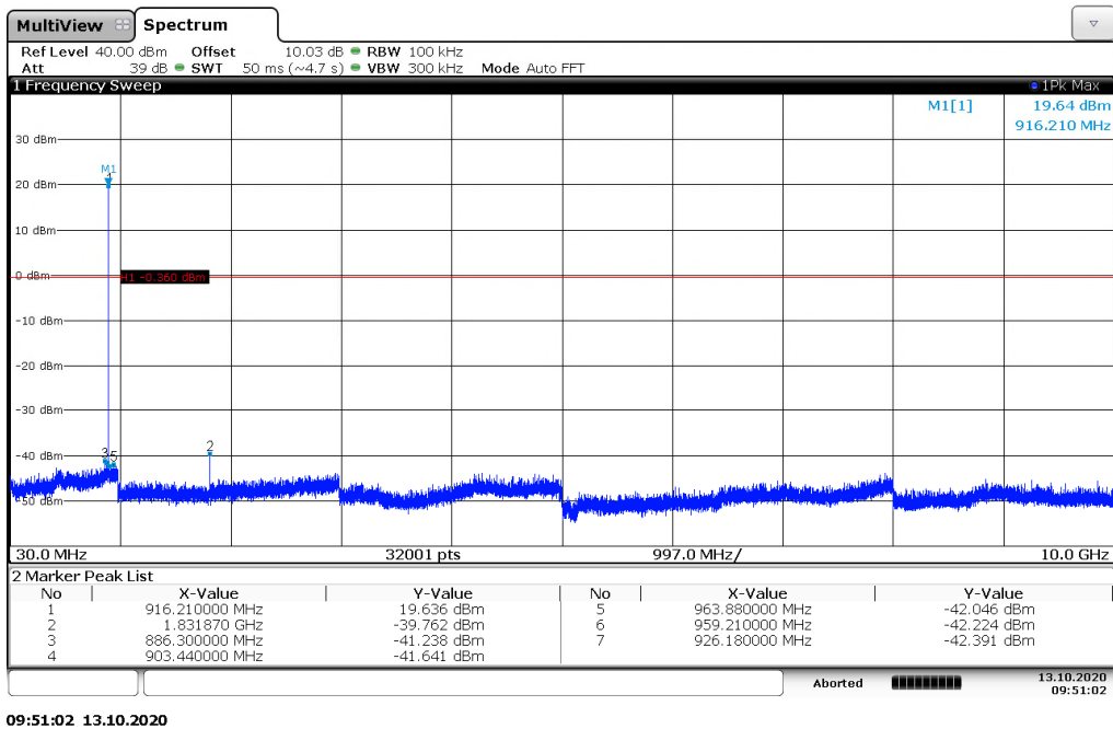
Figure 7.5.2.2-2: 30 MHz – 10 GHz – Mid Channel – 35.5kbps
