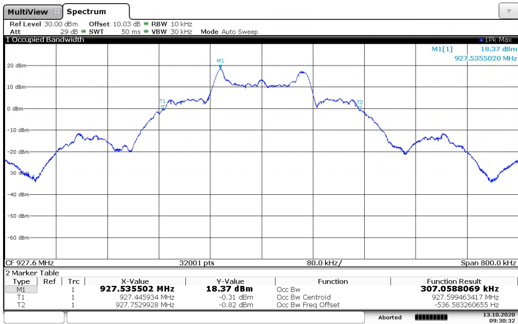
Figure 7.4.4.2-11: 99% OBW High Channel – 142.2kbps
