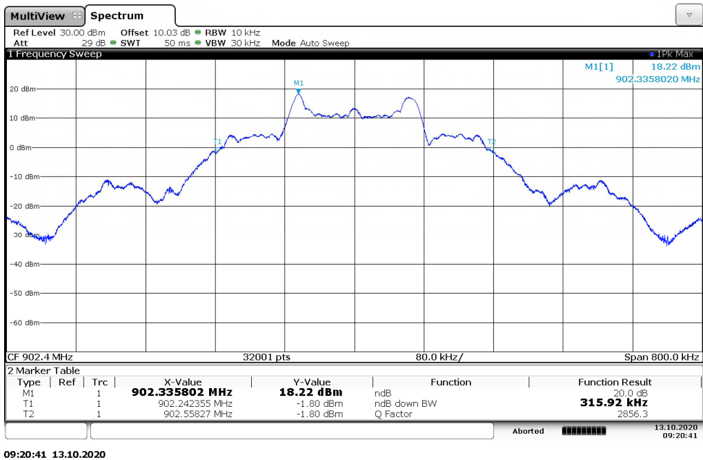
Figure 7.4.4.2-6: 20dB BW Low Channel – 142.2kbps
