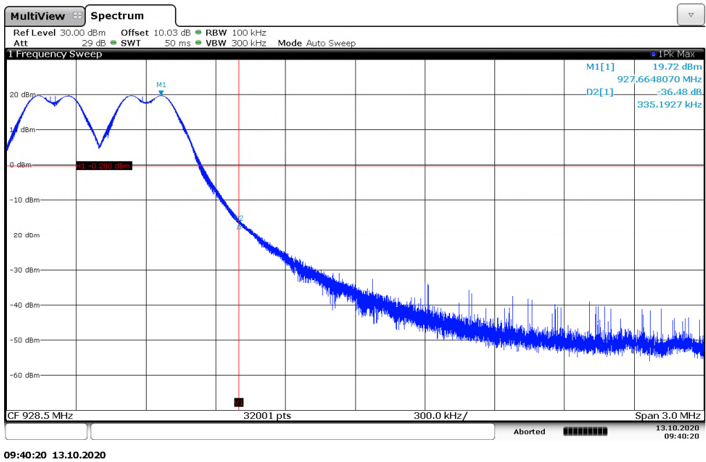
Figure 7.5.1.2-8: Upper Band-edge – 142.2kbps
