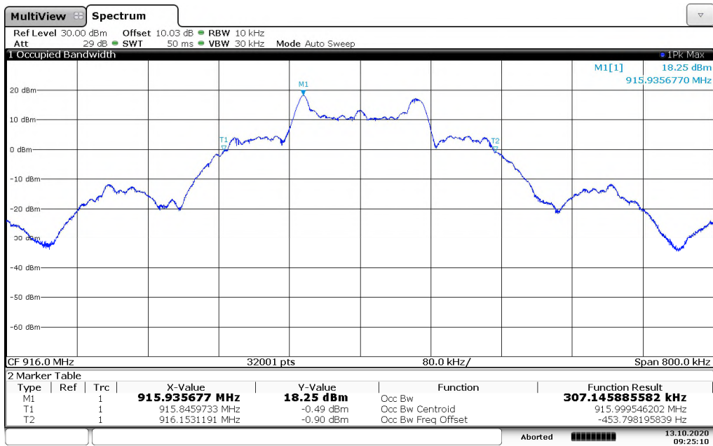
Figure 7.4.4.2-9: 99% OBW Mid Channel – 142.2kbps
