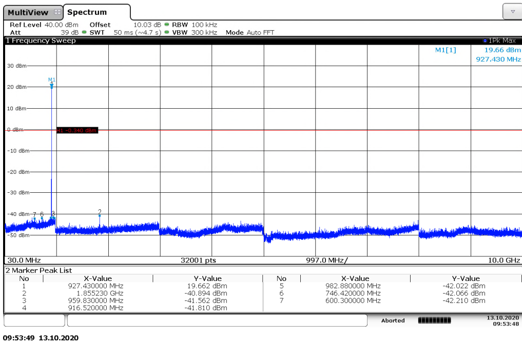
Figure 7.5.2.2-3: 30 MHz – 10 GHz – High Channel – 35.5kbps
