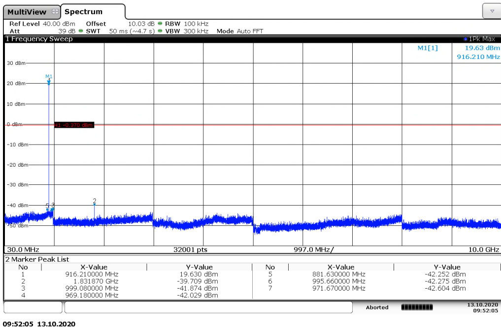
Figure 7.5.2.2-5: 30 MHz – 10 GHz – Mid Channel – 142.2kbps
