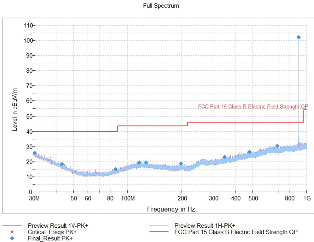
Figure 7.5.3.3-1: Radiated Spurious Emissions Prescan – 30MHz to 1GHz
