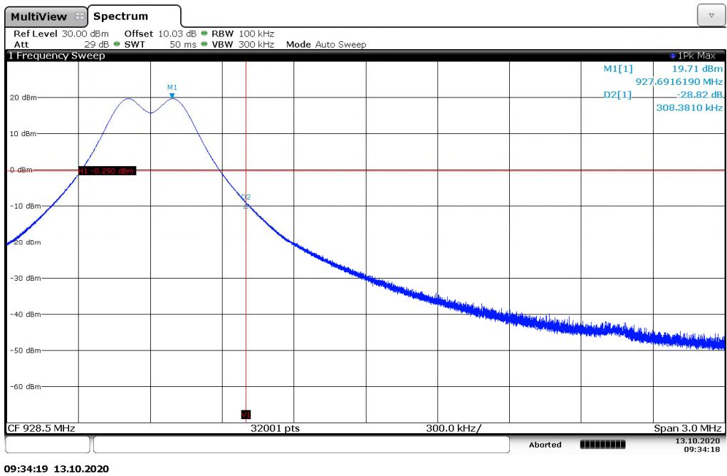
Figure 7.5.1.2-2: Upper Band-edge – 35.5kbps
