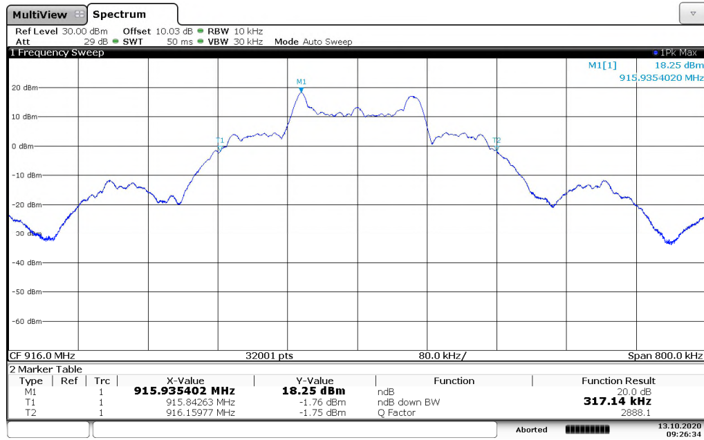
Figure 7.4.4.2-8: 20dB BW Mid Channel – 142.2kbps
