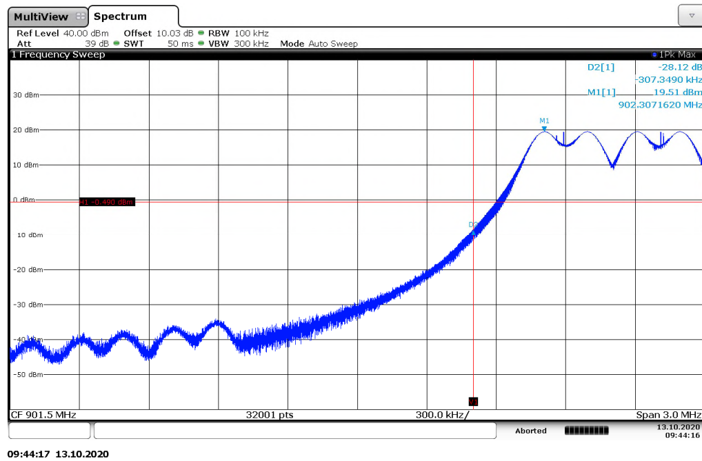
Figure 7.5.1.2-5: Lower Band-edge – 35.5kbps
