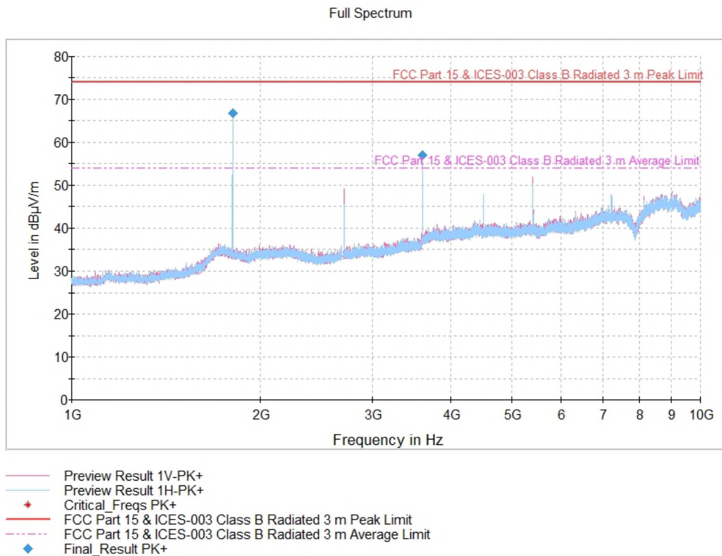
Figure 7.5.3.3-2: Radiated Spurious Emissions Prescan – Above 1GHz
