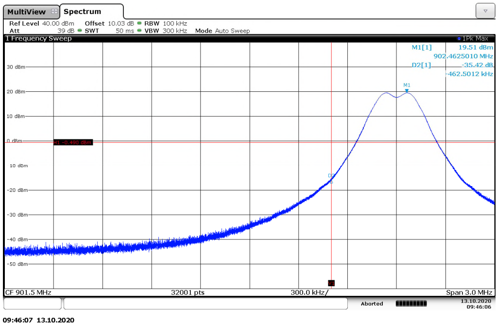
Figure 7.5.1.2-3: Lower Band-edge – 142.2kbps
