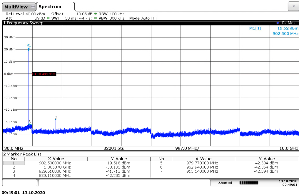
Figure 7.5.2.2-4: 30 MHz – 10 GHz – Low Channel – 142.2kbps
