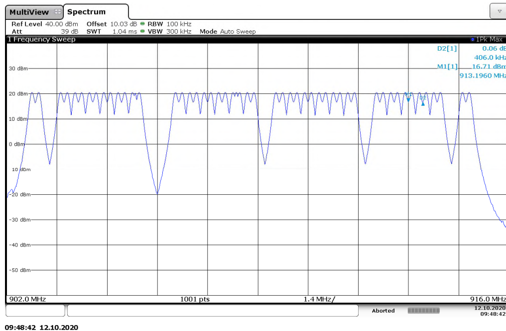
Figure 7.4.2.2-1: Number of Hopping Channels – 35.5kbps
