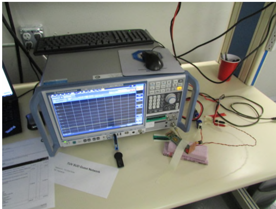
Figure 8: RF Conducted Measurements
