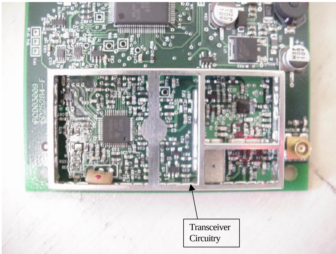
Transceiver.
