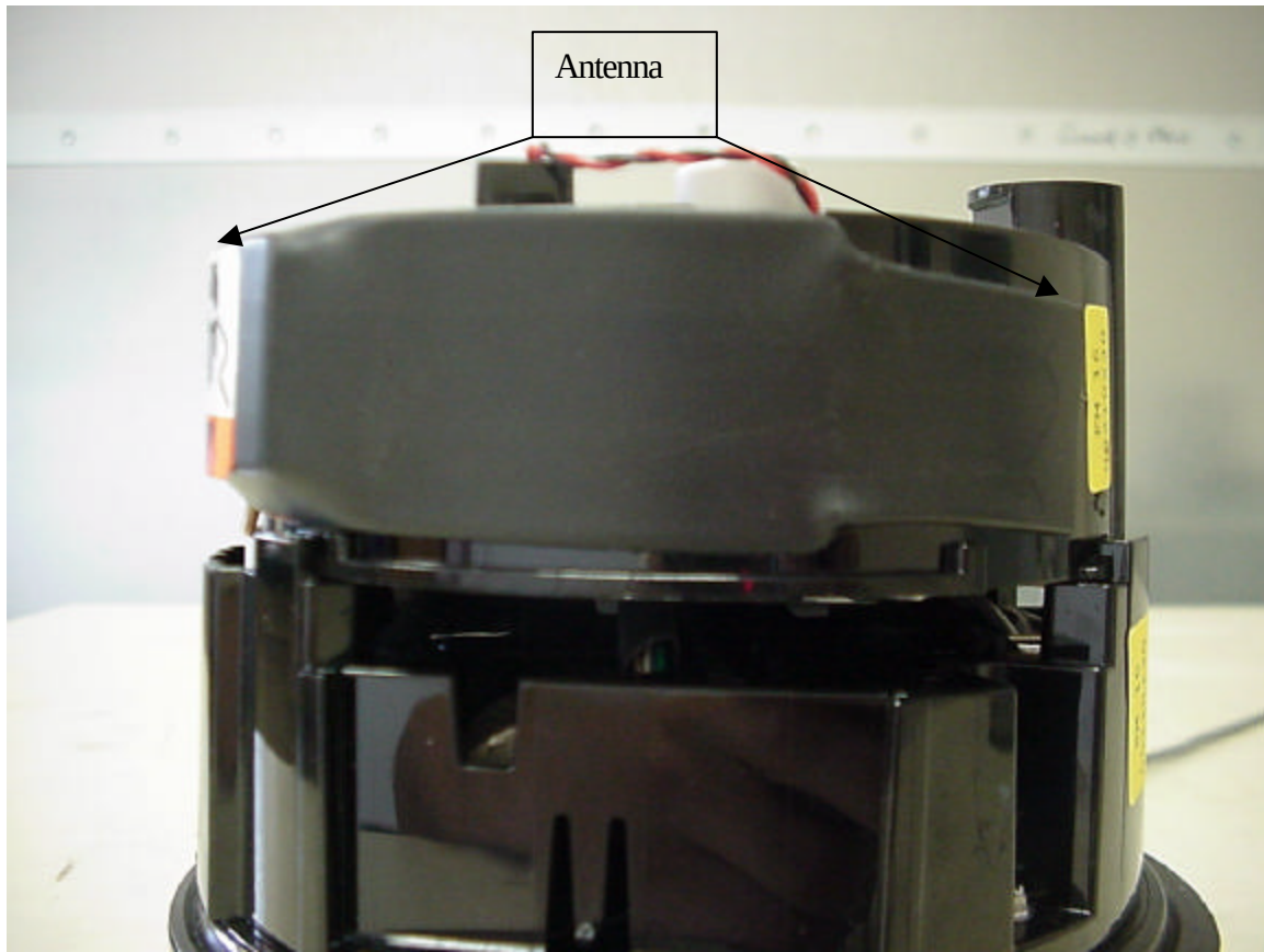
EUT with outer shell removed.
