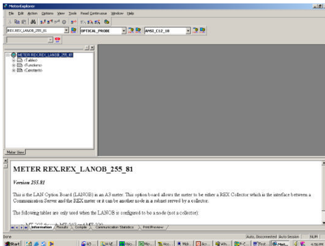
Figure 7: MeterExplorer GUI
