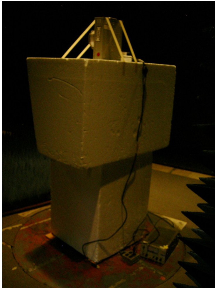
Figure 3: Radiated Emissions
