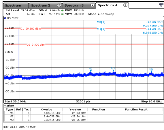
Figure 7.5.2.2-14: 30 MHz – 10 GHz – MCH – 200kbps
