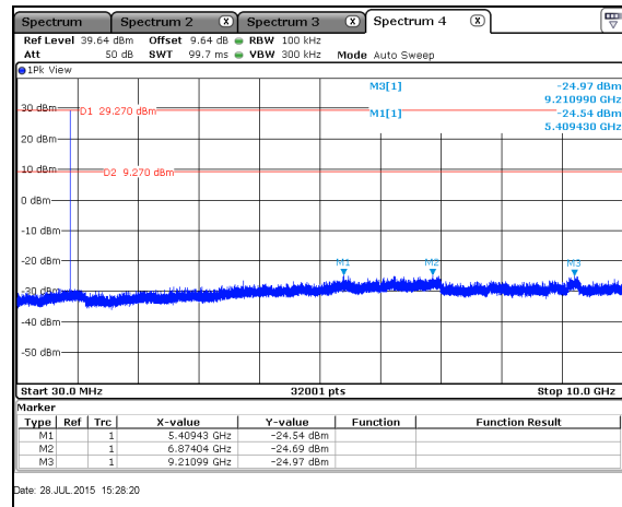
Figure 7.5.2.2-10: 30 MHz – 10 GHz – LCH – 150kbps
