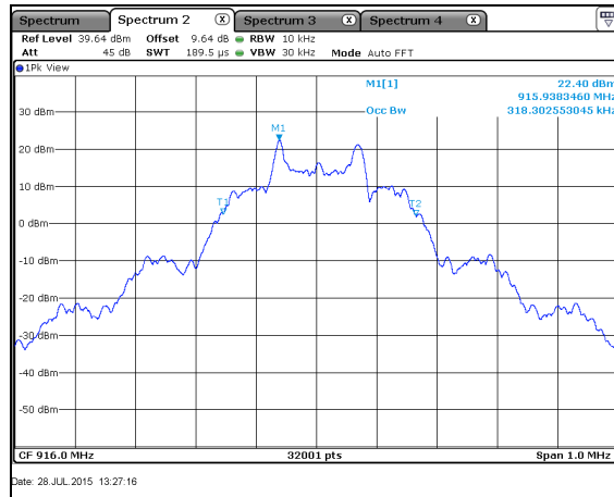
Figure 7.4.4.2-22: 99% BW Mid Channel – 142.2kbps
