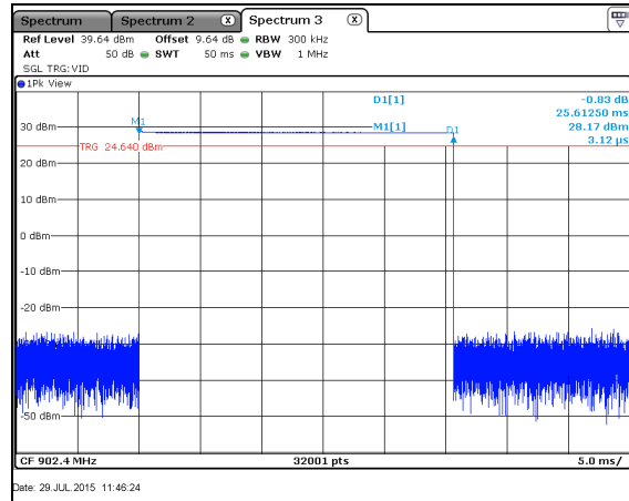
Figure 7.4.3.2-2: Dwell Time – Mode 2
