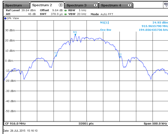
Figure 7.4.4.2-24: 99% BW Mid Channel – 150kbps
