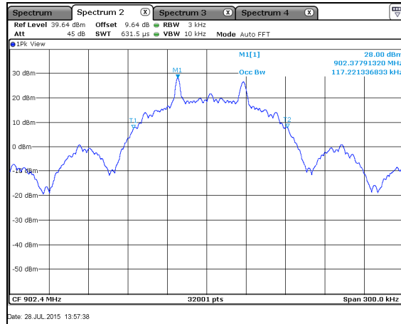
Figure 7.4.4.2-18: 99% BW Low Channel – 50kbps
