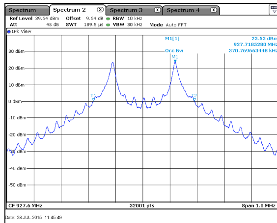
Figure 7.4.4.2-26: 99% BW High Channel – 35.5kbps
