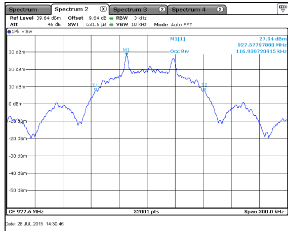
Figure 7.4.4.2-28: 99% BW High Channel – 50kbps
