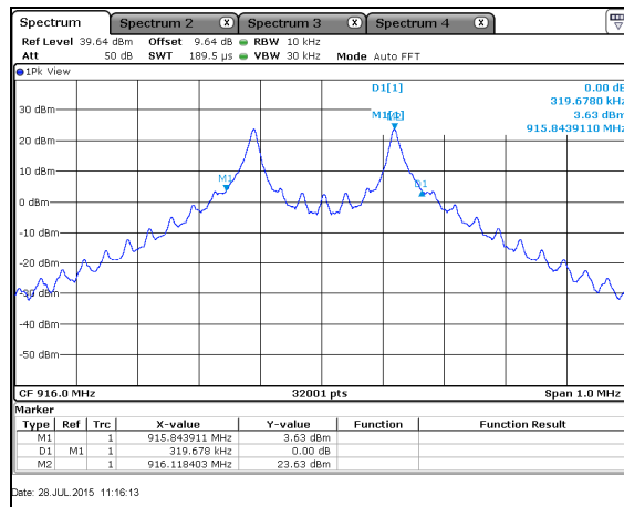
Figure 7.4.4.2-6: 20dB BW Mid Channel – 35.5kbps
