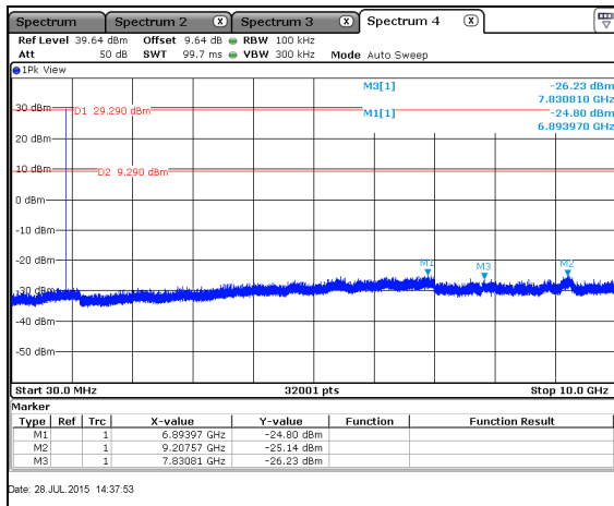
Figure 7.5.2.2-9: 30 MHz – 10 GHz – HCH – 50kbps
