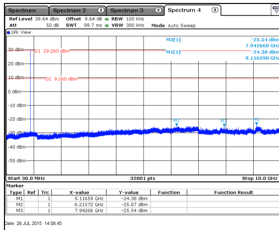
Figure 7.5.2.2-7: 30 MHz – 10 GHz – LCH – 50kbps
