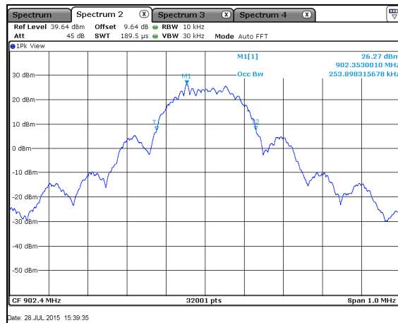
Figure 7.4.4.2-20: 99% BW Low Channel – 200kbps
