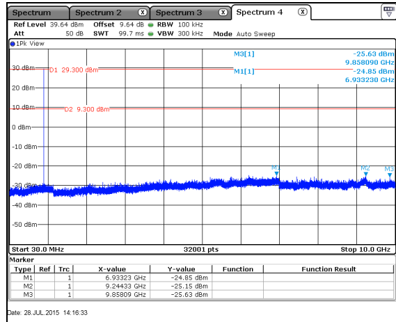
Figure 7.5.2.2-8: 30 MHz – 10 GHz – MCH – 50kbps
