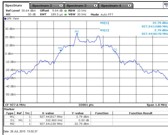
Figure 7.4.4.2-12: 20dB BW High Channel – 142.2kbps
