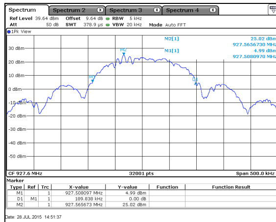
Figure 7.4.4.2-14: 20dB BW High Channel – 150kbps
