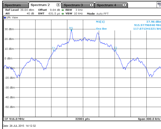
Figure 7.4.4.2-23: 99% BW Mid Channel – 50kbps
