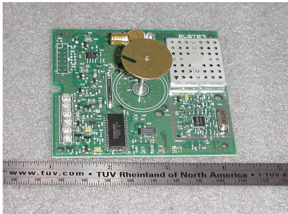
Figure 1 – Top view of circuit board (Shown modified with SMA connector for direct measurements)
