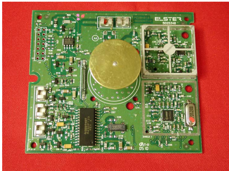
Figure 2 – Top view of circuit board w/o shielding and SMA connector. (Photo provided by manufacturer)
