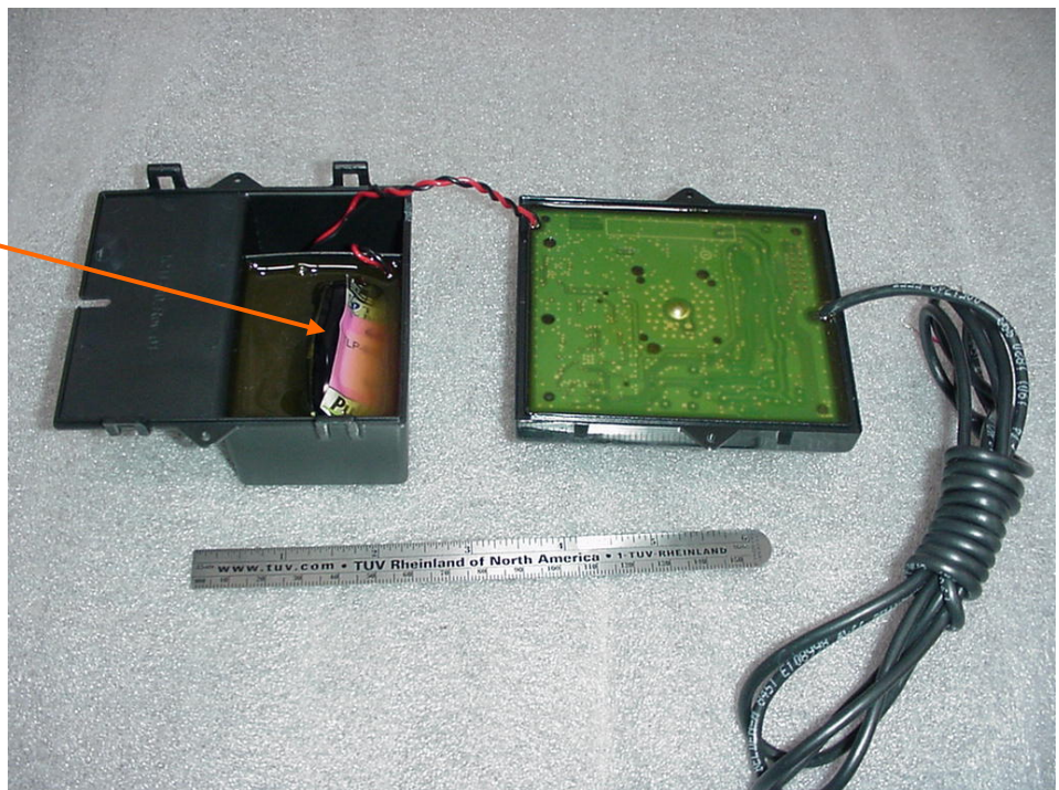
Figure 4 – Internal view of un-modified EUT
